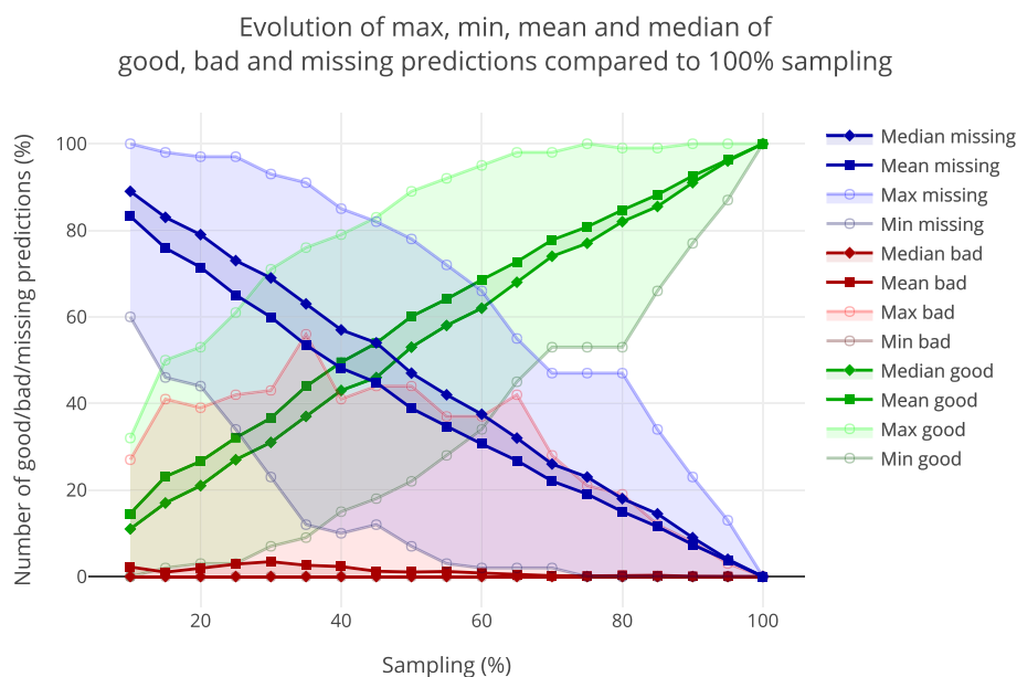
Fig. 3 Stability of the predictions for subsets of observations. This figure summarizes the stability of the predictions for all samplings of the observations, compared to the final predictions with all 100% of observations. “Good” predictions (matching the 100% predictions) are depicted in green, “Bad” predictions (predicted differently than the 100% predictions) in red and “Missing” predictions (not predicted) in blue. For each category, four curves are plotted representing, from top to bottom, the maximum, median, mean and minimum number of predictions of this type. Curves are normalized to the number of predictions obtained for each set of sampled data
