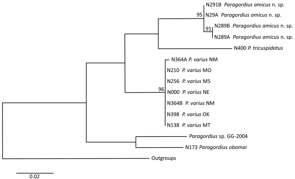
Figure 6. Relationships inferred by maximum likelihood. Tree is unrooted, and drawn to scale indicating number of substitutions per site. Bootstrap values above 0.90 are shown.
