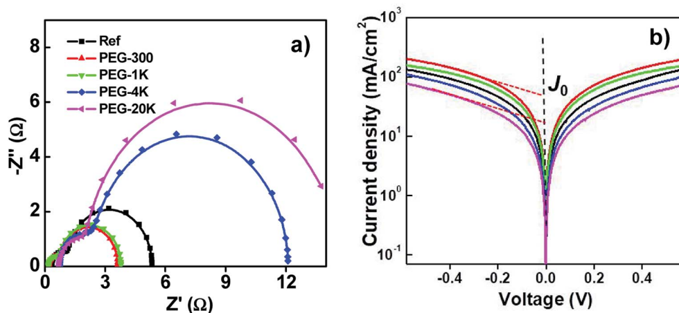
Fig. 3 Electrochemical characterizations of symmetric dummy cells corresponding to electrolyte containing different PEG additives: (a) Nyquist curves, (b) Tafel polarization curves.
