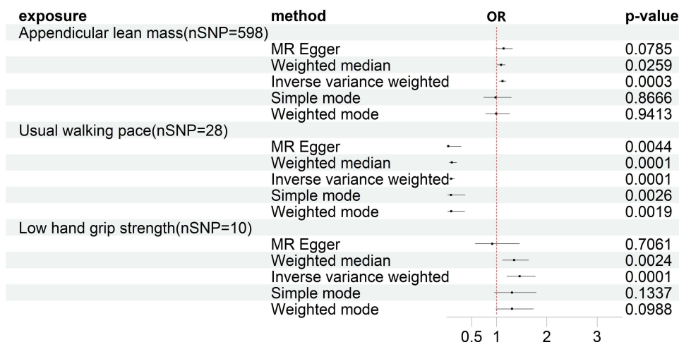
Figure 2 Forest plot of Mendelian randomization analyses. Influence of sarcopenia-related traits on KOA after removing outliers. Abbreviation: OR, odds ratio.
