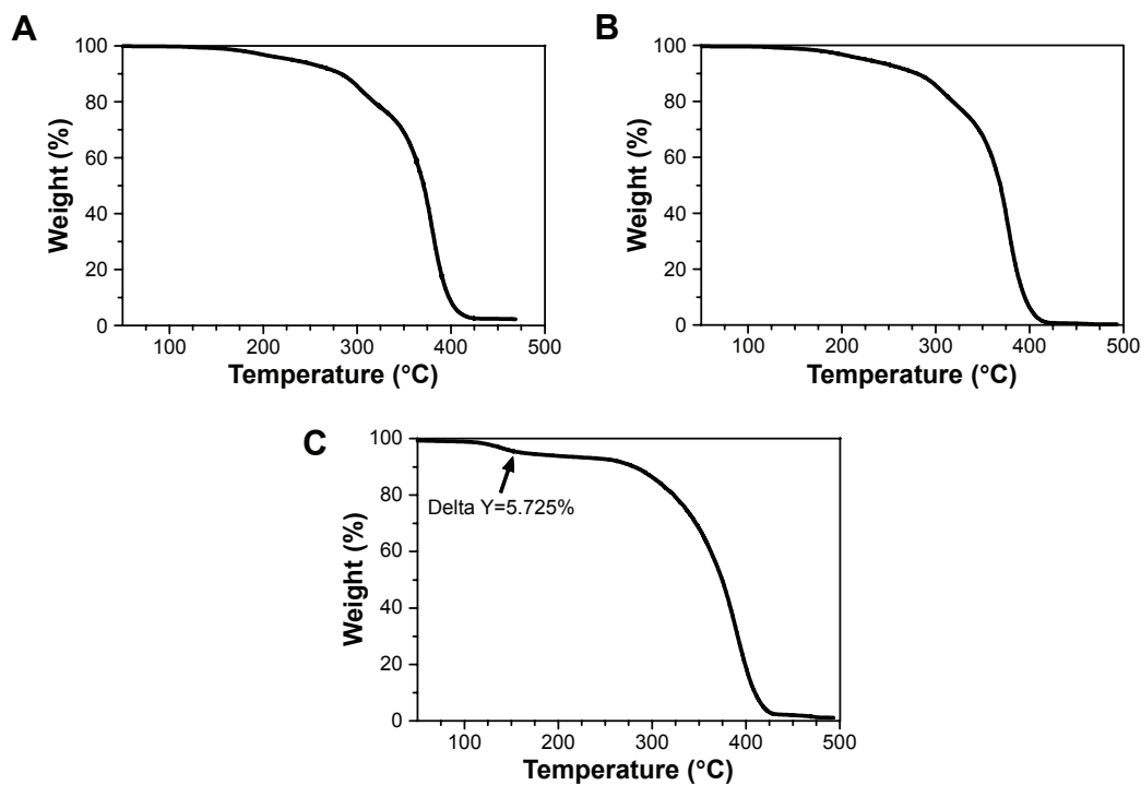
Figure 3 TGA thermogram of PMMA nanoparticles: (A) PMMA-SDS, (B) PMMA-RML, and (C) PMMA-RML-PCA-HEX.
