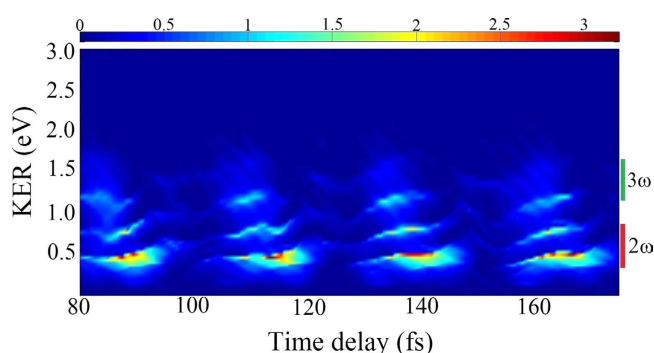
Figure 4. Dependence of the KER spectra on time delay. The red and green bars on the right of the panel indicate the regions of two-net-photon and three-photon dissociation channels, respectively. The laser parameters are the same as in Fig. 2.
