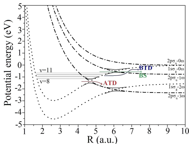
Figure 5. Potential energy curves of \text{H}_2^+ labeled with the net number of absorbed photons ( n\omega ) of wavelength 1600 nm. The solid lines represent the adiabatic anticrossing in Floquet theory, whereas the dotted and dot-dashed lines denote the laser-dressed diabatic potential curves. The horizontal lines represent the vibrational levels, v = 8 \sim 11 . The dissociation channels of ATD, BS, and BTD are indicated by the red, green, and blue arrows, respectively.
