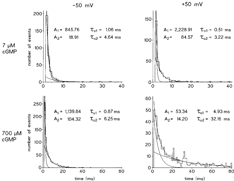
Figure 3. Open-time histograms at 7 and 700 \mu\text{M} cGMP and +50 and -50 mV each. The data were obtained from a multi-channel patch at 7 \mu\text{M} cGMP and a single-channel patch at 700 \mu\text{M} cGMP. The distributions were fitted with sums of two exponentials yielding the indicated contributions A_n and open-time constants \tau_n . The combination of high [cGMP] and positive voltage caused a dramatic prolongation of both time constants. Filter, 2 kHz.
