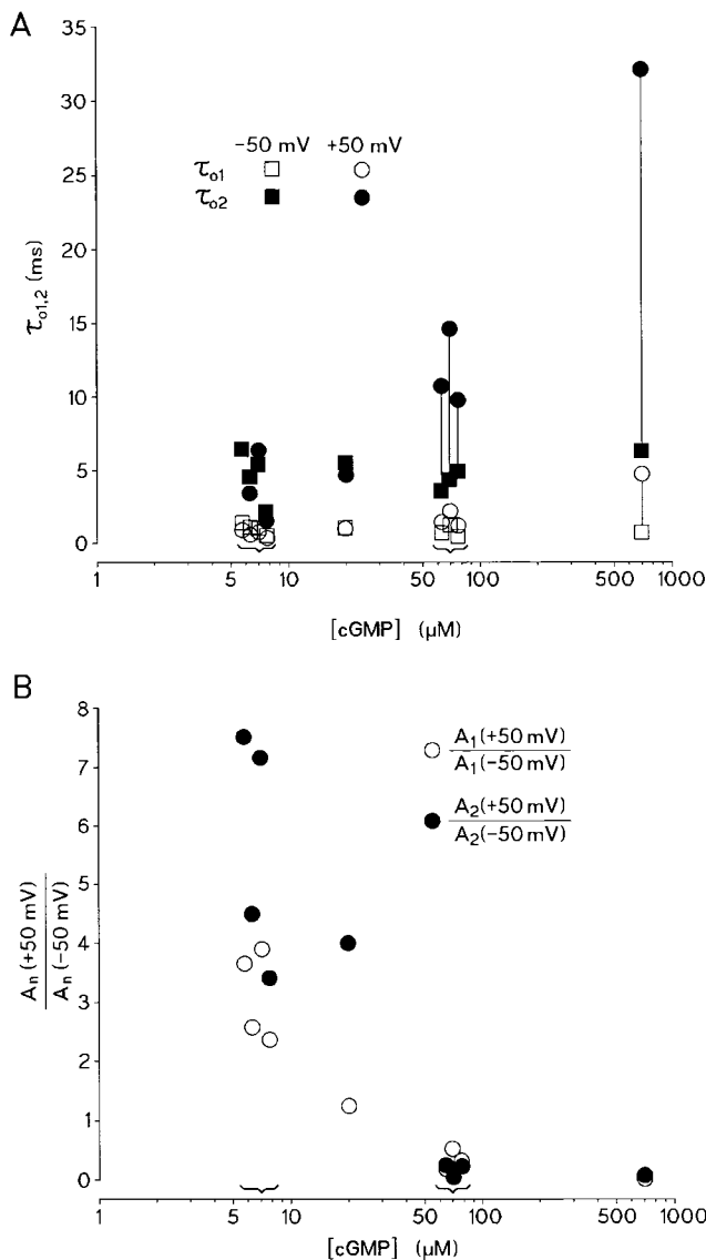
Figure 4. Dependence of open times on [cGMP]. All data were filtered at 2 kHz. (A) Fast open time \tau_{o1} and slow open time \tau_{o2} of single cGMP-gated channels as function of [cGMP]. Kinetic constants were measured at 7, 20, 70, and 700 \mu\text{M} cGMP and at -50 and +50 mV. Parentheses indicate values at 7 and 70 \mu\text{M} , respectively. 16–63 traces of 500-ms duration were analyzed. When switching from -50 to +50 mV, both \tau_{o1} and \tau_{o2} increased at 70 \mu\text{M} cGMP and even more so at 700 \mu\text{M} cGMP, whereas at 7 and 20 \mu\text{M} cGMP, no statistically significant increase of either \tau_{o1} and \tau_{o2} was observed. (B) Voltage-dependent incidence of the relative contribution of fast and slow exponential in the open-time histograms as function of [cGMP]. Plotted is the ratio A_n(+50\text{ mV})/A_n(-50\text{ mV}) . At low [cGMP], A_2(+50\text{ mV})/A_2(-50\text{ mV}) is larger than A_1(+50\text{ mV})/A_1(-50\text{ mV}) , suggesting that the contribution of the slow exponential is more influenced by voltage than that of the fast exponential.
