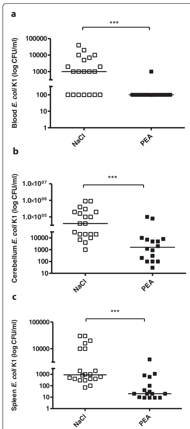
Figure 5 Bacterial concentrations in spleen, blood and cerebellum after intracerebral infection. Bacterial concentrations (CFU/ml) in blood (a), cerebellum (b) and spleen (c) 24 hours after intracerebral E. coli infection. Statistical analysis was performed by Mann-Whitney U -test. Data are shown as individual measurements and medians (***) P < 0.001 .
