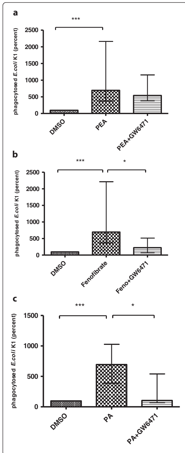
Figure 2 Involvement of peroxisome proliferator-activated receptor (PPAR)α in macrophage stimulation and phagocytosis of E. coli K1 by palmitoylethanolamide (PEA), fenofibrate and palmitic acid (PA). Macrophages were incubated with the PPARα antagonist GW6471 (1 μM) for 1 hour. After incubation, macrophages were either left unstimulated (treated with medium containing 0.01% DMSO) or stimulated with PEA (300 nM) (a), fenofibrate (20 μM) (b) or palmitic acid (PA) (0.25 mM) (c) for 1 hour (n ≥ 9 wells/group from two independent experiments). In each experiment, the number of bacteria ingested by the control group (DMSO) was considered to be 100%. Phagocytic rates are presented as the percentage of phagocytosis of the respective control group. Data are given as medians with interquartile ranges and were analyzed by Kruskal-Wallis test followed by Dunn's correction for repeated testing (** P < 0.001, * P < 0.05).
