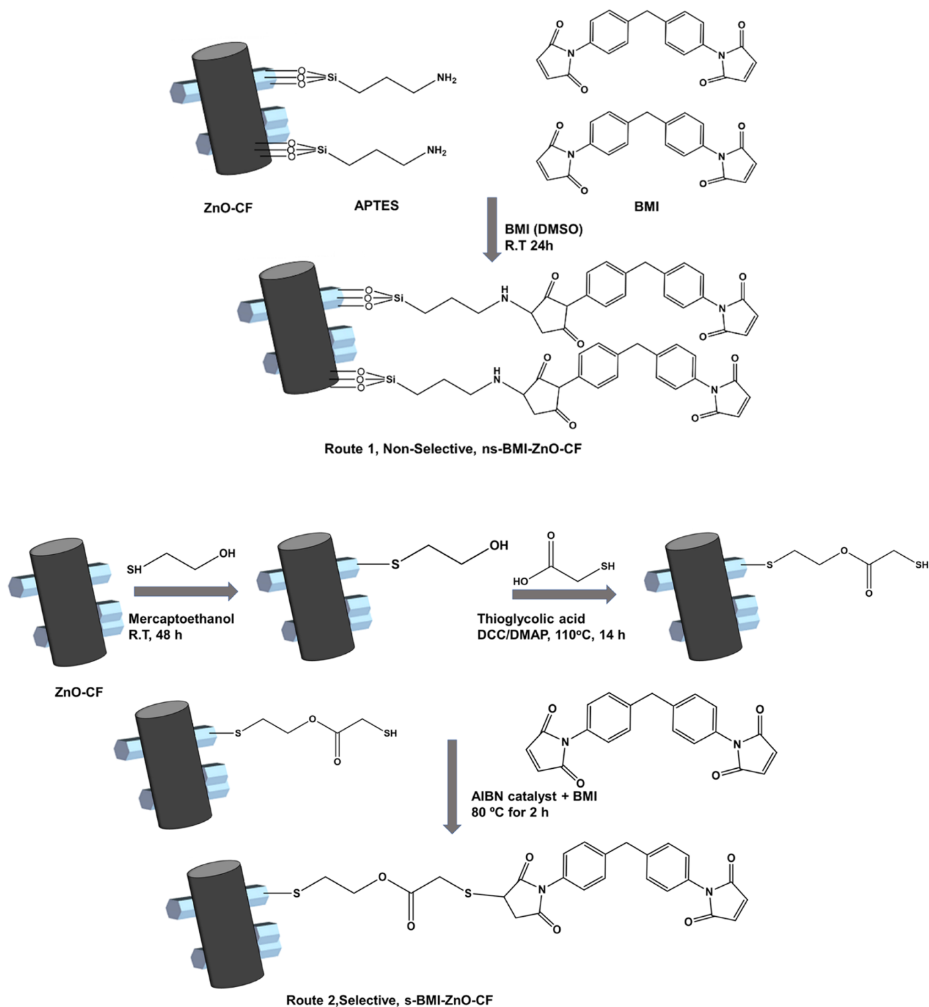
Figure 1. Chemical routes to attach BMI on ZnO–CF. Route 1 indicates nonselective deposition and route 2 indicates selective deposition of BMI.
