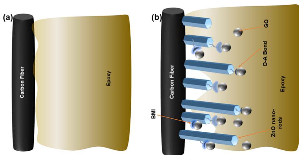
Figure 10. CF–epoxy interfacial scheme for (a) neat and (b) modified laminates with fiber and matrix modification.
