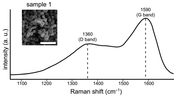
FIG. 3. Raman spectroscopy of the fossil soft tissues. Merged spectrum of three measurements of sample 1. Raman peaks at c. 1360 and 1590 \text{cm}^{-1} represent kerogen D and G bands, respectively. SEM micrograph on the top left corner is sample 1, Region 1. Scale bar represents 2 \mu\text{m} .
