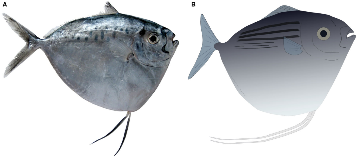
FIG. 5. Evolution of menid colour patterns. A, the extant moonfish Mene maculata . B, schematic reconstruction of the Eocene Mene rhombea based on evidence for countershading and longitudinal dorsal stripes. The length of the anal fins is estimated based on data available for fossil and extant taxa.
