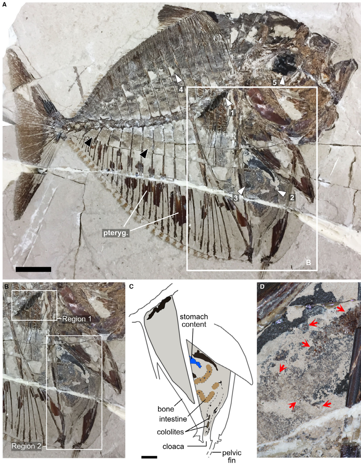
FIG. 1. Soft tissues and stomach content of the fossil moonfish. A, MCSNV 18/2020 (part) Mene rhombea (Menidae); the brown-coloured material present ventrally corresponds to the remains of the anal fin bones (pterygiophores; pteryg.); white triangles and associated numbers indicate sampling locations; black triangles indicate the most ventral evidence of the integument. B–C, detail of the abdomen showing stomach contents, cololites, and preservation of the gut as carbonaceous material; C, schematic representation with soft tissue interpretation. D, detail of the abdomen of the counterpart MCSNV 19/2020 showing the upper part of Region 2, illustrating the stomach and intestine (see Fig. S1); red arrows indicate the vertebrae and other ingested bones of clupeid fish. Scale bars represent: 20 mm (A); 10 mm (B, C).
