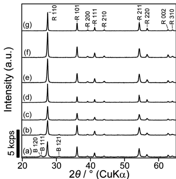
Fig. 1 XRD patterns of (a) meso-TiO 2 , (b) meso-N-TiO 2 , (c) meso-N-TiO 2_873 , (d) template free-TiO 2 , (e) template free-N-TiO 2 , (f) template free-N-TiO 2_873 , and (g) template free-N-TiO 2_1173 . The peaks marked as B and R are assigned to the brookite and rutile phases, respectively.
