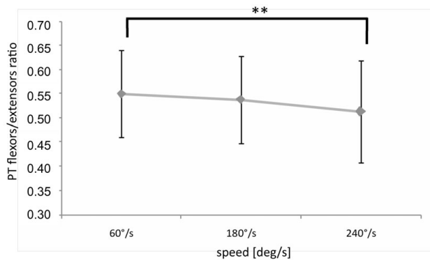
Figure 1 Speed main effect on flexors/extensors ratio: estimated marginal means and post-hoc analysis. ** p < 0.01.
