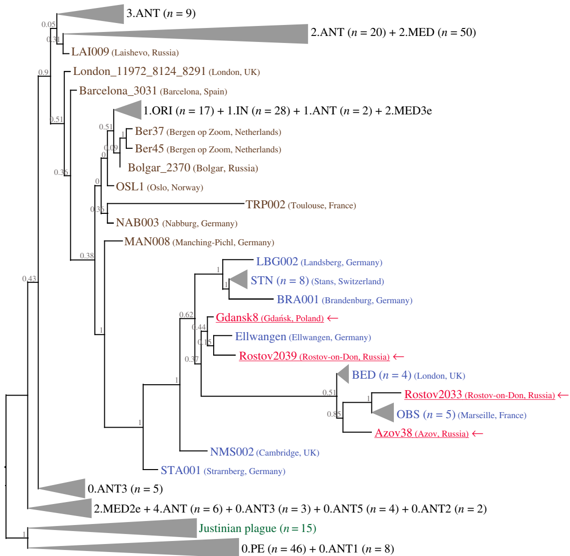
Figure 2. Maximum-likelihood tree (RAxML) showing the location of ancient Y. pestis genomes among main Y. pestis clusters. The newly studied Y. pestis genomes (fifteenth to eighteenth century) are in red and marked by arrows. The previously published samples closer to the Black Death period (thirteenth to fourteenth century, [12,20,27]) are marked in brown. The previously published samples dated to the post-Black Death period (fifteenth to eighteenth century, [18,20,27]) are marked in blue. The samples from the first epidemic (sixth century, [34]) are marked in green. The modern Y. pestis strains and first plague epidemic samples are collapsed to improve the tree visibility. The number of samples inside the collapsed branches are indicated in brackets. For detailed information about modern branches, see electronic supplementary material, table S2 and figure S3. Node labels are bootstrap support (100 iterations). Yersinia pseudotuberculosis genome [43] was used as an outgroup. For the complete phylogenetic tree, see electronic supplementary material, figure S3. (Online version in colour.)
