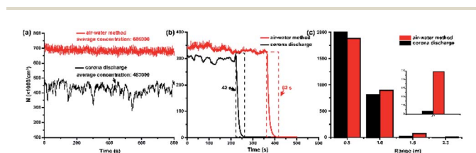
Fig. 2 Comparison of physical properties of NAIs prepared by corona discharge and air–water collision with rosin-TiO 2 . (a) Average intensity and stability of ENAIs and HNAIs; (b) lifetime of ENAIs and HNAIs at same density; (c) straight propagation distance of ENAIs and HNAIs. All experiments were performed at room temperature in laboratory (March, 2018, Beijing).
