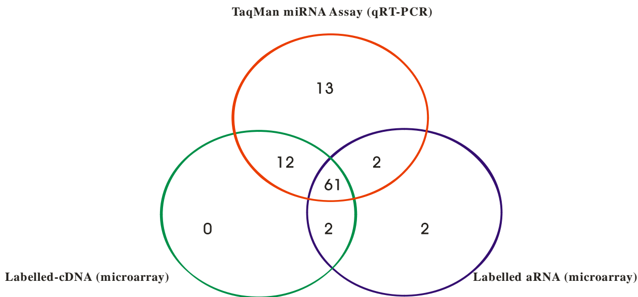
Figure 6 Venn diagram to illustrate miRNAs detected by TaqMan ® MiRNA Assay quantification and miRNA microarray analysis.
