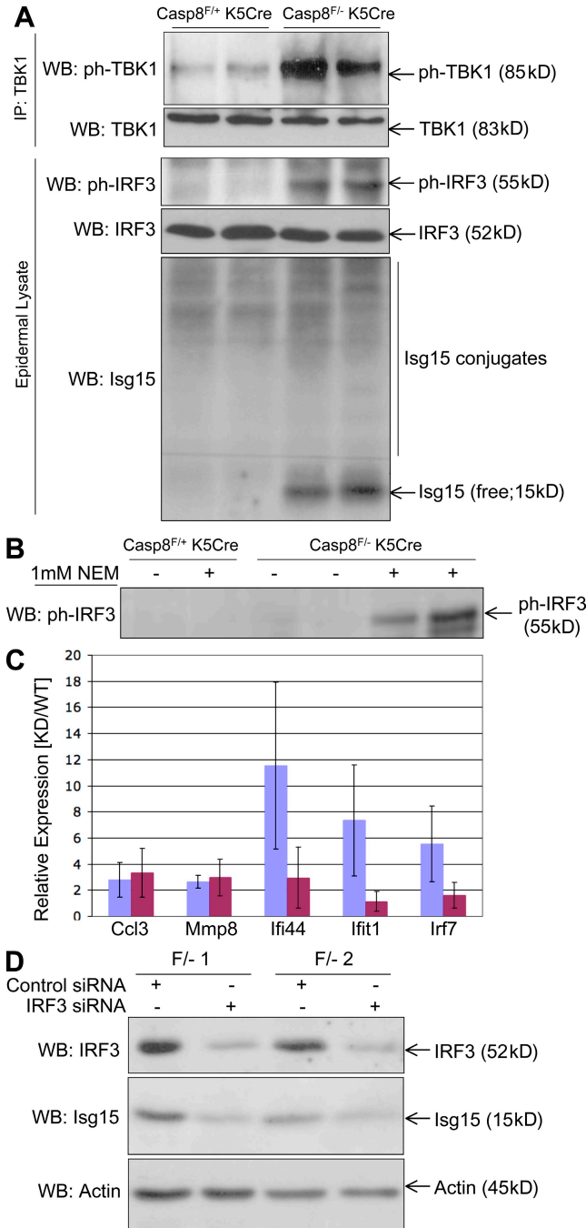
Figure 7. IRF3 is constitutively activated in the Casp8 -/- K5-Cre epidermis. (A) Western blot analysis of lysates of the epidermis of two Casp8 +/+ K5-Cre and two Casp8 -/- K5-Cre littermates at P3 for phosphorylation of TBK1 (ph-TBK1, enriched by immunoprecipitation with anti-TBK antibody) and of IRF3 (ph-IRF3), as well as for expression of IRF3 and of the IRF3-induced protein Isg15, and conjugation of Isg15 to the cellular proteins. (B) Western analysis of ph-IRF3, as in A, for mouse littermates at P1. As illustrated, the small amount of ph-IRF3 in the lysates of the Casp8 -/- K5-Cre epidermis at that date could be discerned only when the cells were lysed in the presence of the sulphhydryl blocking agent N -ethylmaleimide. (C and D) Activation of inflammatory genes in early passage Casp8 -/- K5-Cre keratinocytes is dependent on the presence of IRF3. (C) Relative expression (means \pm SD of the indicated gene transcripts in Casp8 -/- K5-Cre mRNA to
