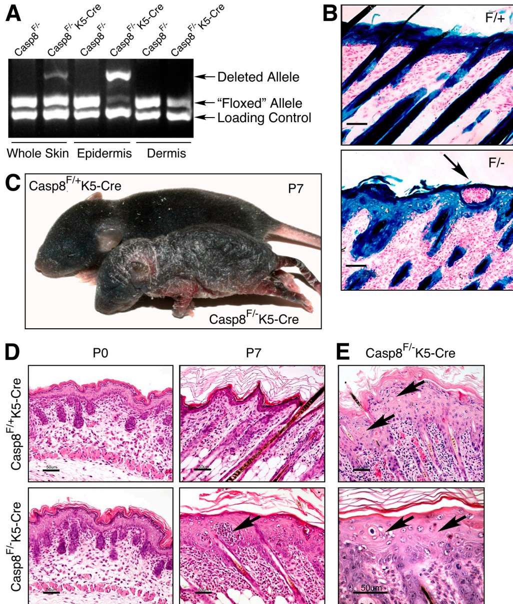
Figure 2. Epidermis-specific KO of caspase-8. (A) Quantitative assessment of WT and deleted caspase-8 alleles in Casp8 F/- K5-Cre mice by genomic PCR. (B) X-gal staining for β-galactosidase activity in the skins of ROSA26-reporter Casp8 F/+ K5-Cre (F/+) and ROSA26-reporter Casp8 F/- K5-Cre (F/-) mice, demonstrating specific Cre-induced recombination in the superficial and follicular epidermis and hair follicles. Bars, 50 μm. (C) General appearance of Casp8 F/+ K5-Cre and Casp8 F/- K5-Cre mice at P7. The mutant is much smaller than the WT. The skin is unevenly thickened with marked alopecia and hyperkeratosis. (D) Microscopy of the skin. At P0, the skin of the Casp8 F/- K5-Cre mice is indistinguishable in appearance from the skin of the Casp8 F/+ K5-Cre mice. At P7 there is marked epidermal hyperplasia and widespread dermal inflammatory cellular infiltration in the Casp8 F/- K5-Cre mouse. Arrows in B and D point to intraepidermal eosinophilic pustules. H&E; Bars, 50 μm. (E) The affected epidermis contains numerous dyskeratotic foci, consisting of maloriented keratinocytes often forming a whorl around a central keratinocyte which has become prematurely keratinized (arrows). H&E; Bars, 50 μm. The data presented in B, C, D, and E are representative of analyses of 4, 350, 30, and 30 mice, respectively.
