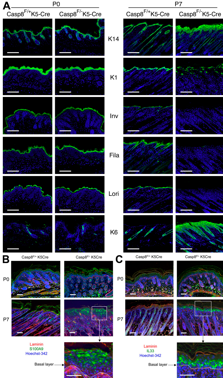
Figure 4. Spatial analysis of the effects of caspase-8 deficiency on protein and gene expression in the epidermis. (A) Immunohistochemical characterization of the caspase-8-deficient epidermis. At P7 (right), immunostaining shows expression of the basal layer marker K14 throughout the Casp-8 F/- K5-Cre epidermis. Staining for the intermediate (K1 and involucrin [Inv]) and late (filaggrin [Fila] and loricrin [Lori]) differentiation markers shows either their disorganized localization or their almost complete absence in the Casp-8 F/- K5-Cre lesion areas. Also shown is the ubiquitous expression of
