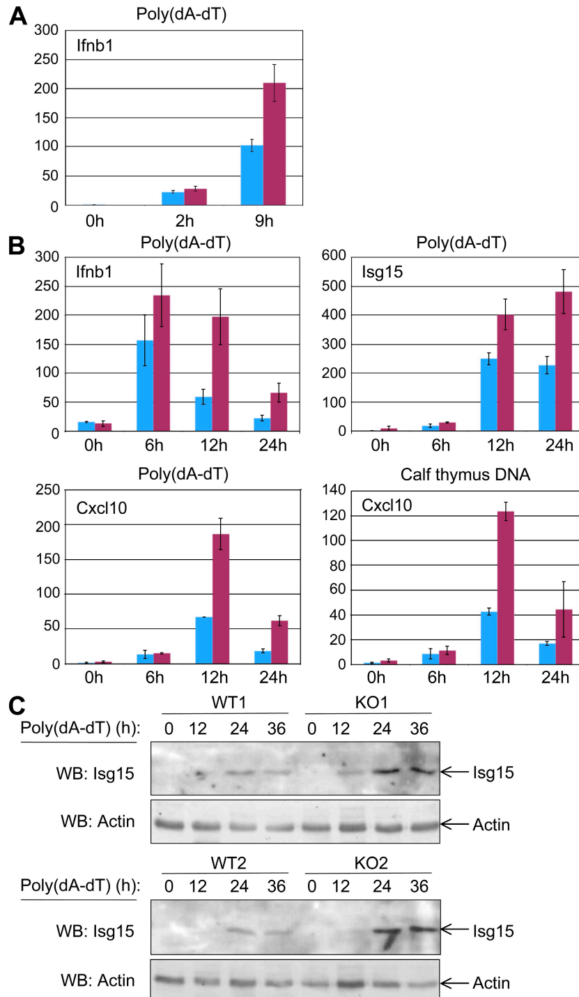
Figure 8. Caspase-8-deficient keratinocytes display an enhanced response to transfected DNA. (A and B) Effect on gene activation. (A) Effect of caspase-8 knockdown. Relative expression of the IFNβ gene (ratio of the IFN-β transcript in caspase-8 knockdown keratinocytes to the same transcripts in mock-transfected cells) assayed in keratinocytes from one pair of P1 littermates that were transfected in duplicate, 1 d after plating, with either control siRNA (blue) or caspase-8 siRNA (maroon) and, 72 h later, transfected with poly(dA-dT) for the indicated times. Shown are mean expression ratios ± SD for the respective duplicate transfections. (B) Effect of caspase-8 KO. Expression of the indicated gene transcripts at different times after DNA transfection of keratinocytes from Casp-8 fl/+ K5-Cre mouse and Casp-8 fl/- K5-Cre mouse epidermis from two pairs of P1 littermates, 1 d after plating. Cells were transfected either with poly(dA-dT) or with calf thymus DNA, as described in Materials and methods. (C) Effect on Isg15 expression. Western analysis of the expression of Isg15 protein at different times after poly(dA-dT) transfection of keratinocytes from Casp-8 fl/+ K5-Cre and Casp-8 fl/- K5-Cre epidermis from two pairs of P1 littermates, 1 d after plating, as in A. Analysis of the expression of β-actin served as a loading control. The data presented in each of the panels are representative of findings obtained in two independent experiments.
