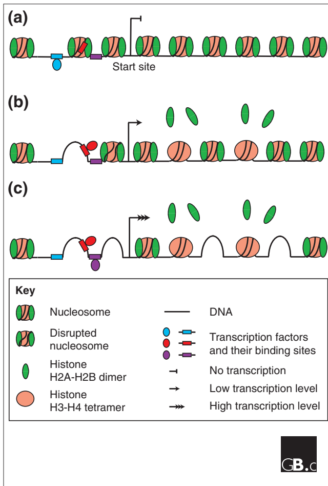
Figure 1 A model for the change in nucleosome occupancy in a typical yeast gene in different transcriptional states. (a) When there is no transcription, repressor proteins bind to their DNA-binding sites and maintain a repressive chromatin configuration with nucleosomes all along the gene and most of the promoter. (b) When activator proteins bind their DNA elements, they promote changes in chromatin that disrupt or displace nucleosomes from promoter regions, leading to transcription of the gene. Subsequent transcript elongation through coding regions causes the transient displacement of histones. (c) With higher levels of transcription, nucleosomes become depleted from coding regions as well as from the promoter.
