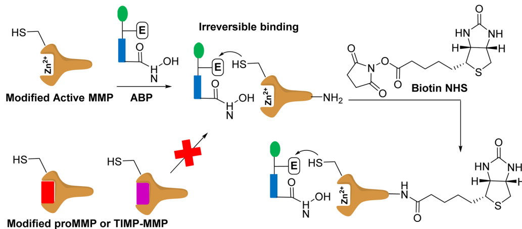
Fig. 5 Modified MMP binds to affinity based probe (ABP). The modified MMP contains a cysteine. The modified active MMP binds to the ABP irreversibly. The proMMP or TIMP-MMP cannot bind to the ABP as the active site is not accessible as the prodomain and TIMP block it. The labelled active MMP can be treated with biotin for protein purification, and subsequent identification.
