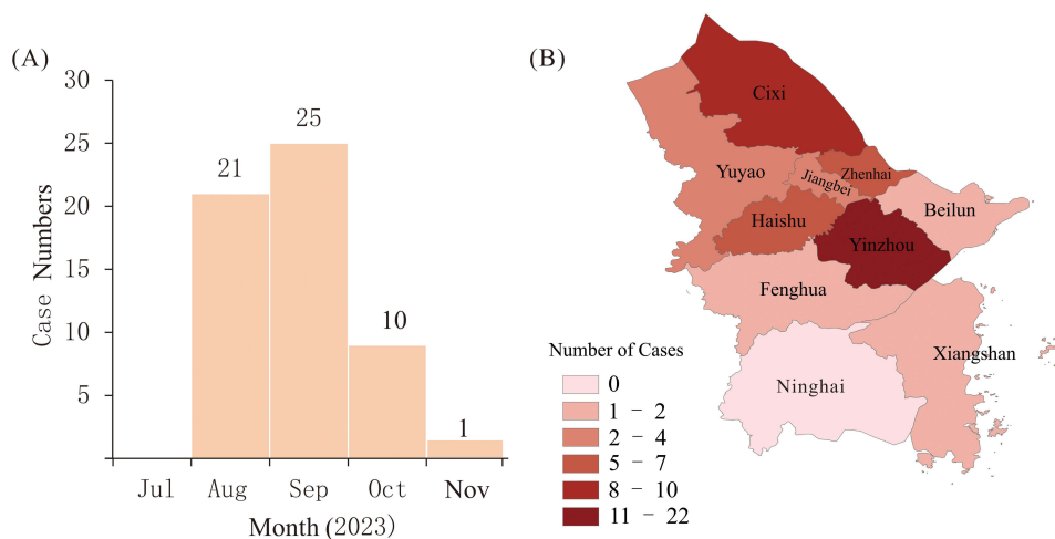
Figure 1 The Temporal and Regional Distribution for Dengue Infections in Ningbo, 2023.
