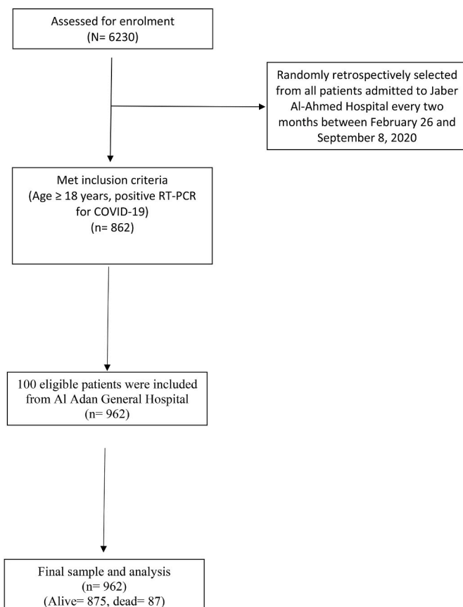
Fig. 1. Study flowchart.
