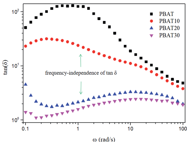
Fig. 9 Plots of \tan \delta versus frequency for the neat PBAT and its blends.
