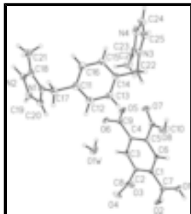
Fig. 1. Fig. 1. The molecular structure of (I), showing displacement ellipsoids at the 30% probability levels.
