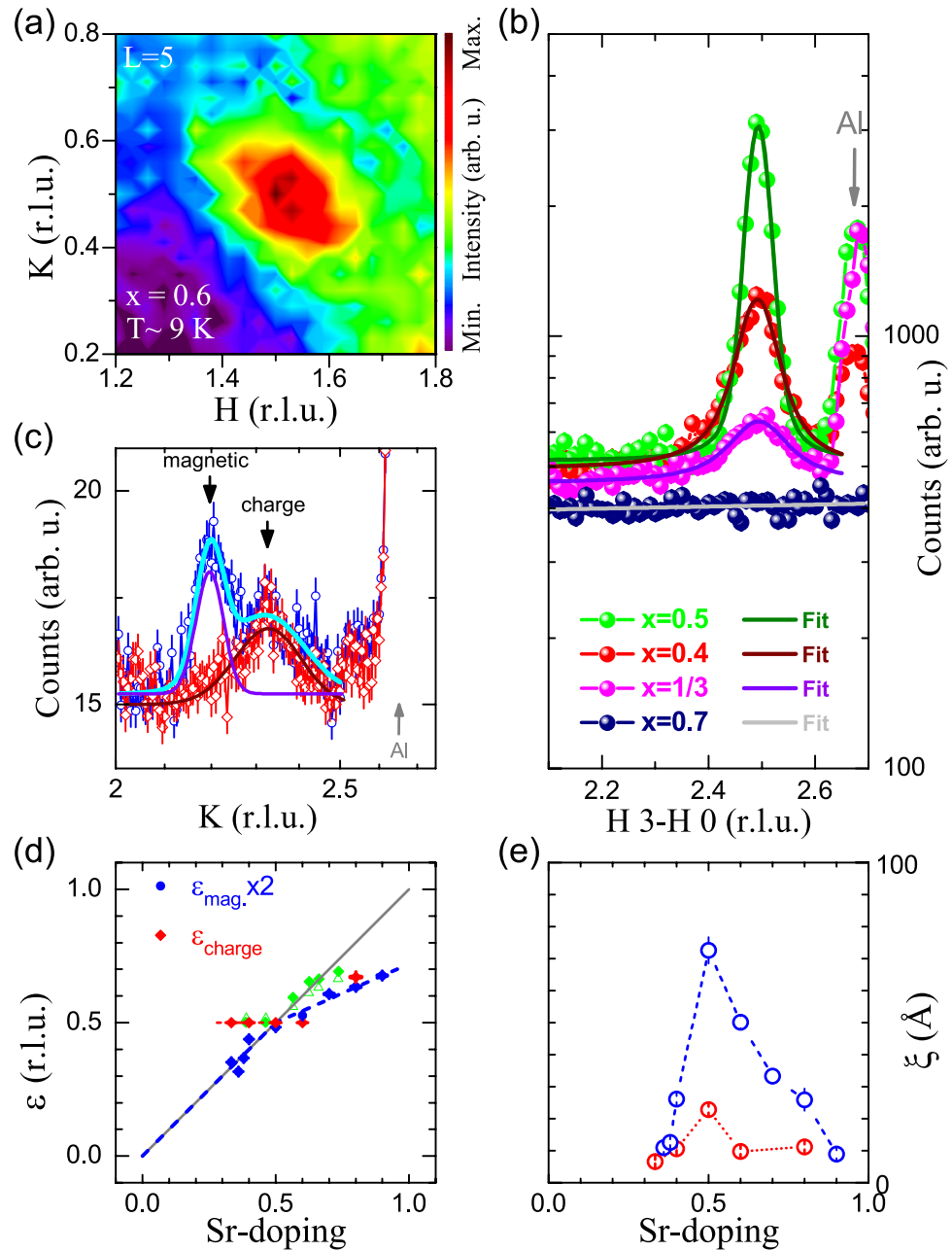
Figure 2. (a) Synchrotron radiation single crystal X-ray diffraction measurements reveal half-integer peaks in La 1.4 Sr 0.6 CoO 4 at ~9 K which are indicative for CBCO. (b) Neutron diffraction measurement of the charge correlations in La 1.3 Sr 0.7 CoO 4 . For direct comparison practically the same experimental conditions as for the study of the half- and underdoped cobaltates with x = 0.5, 0.4 and 1/3 published in ref. 17 were reproduced. (c) Neutron scattering intensities measured in a diagonal ( 3 - K K 0 ) scan for the sample with x = 0.8 at ~3 K (blue) and 100 K (red). As can be seen, the charge correlations are incommensurate at such high hole-doping. The magnetic and charge ordering peak positions at 3 K were determined by fitting two Gaussians (cyan dotted line), and they equal 2.196(3) and 2.320(15), respectively. The charge ordering peak position at 100 K (solid magenta line) is 2.329(5). The corresponding incommensurabilities for charge and magnetic peaks are 2 \cdot \epsilon_{\text{mag}} = 0.608(6) , \epsilon_{\text{charge}}(3 \text{ K}) = 0.680(15) , and \epsilon_{\text{charge}}(100 \text{ K}) = 0.671(5) . (d) Sr-doping dependence of the charge and magnetic incommensurabilities, 2 \cdot \epsilon_{\text{mag}} and \epsilon_{\text{charge}} , respectively. Green data points are the corresponding values for Pr 2-x Ca x CoO 4 taken from ref. 24; open/closed symbols: 2 \cdot \epsilon_{\text{mag}}/\epsilon_{\text{charge}} . (e) The correlation lengths \xi_{\perp \vec{q}} (blue: magnetic; red: charge) for different values of x . Here, the \xi_{\perp \vec{q}} are greater than \xi_{\parallel \vec{q}} (e.g. 59(19)% greater for x = 0.7 ). It should be noted that \xi_{\perp \vec{q}} and \xi_{\parallel \vec{q}} are defined as the correlation lengths perpendicular and parallel, respectively, to the direction of \vec{q} with incommensurate magnetic peak positions \vec{q} = \vec{Q}_{\text{inc}} - (1/2 \ 1/2 \ 0) and \vec{Q}_{\text{inc}} , respectively. The correlation lengths were obtained from the inverse of the (Lorentzian) peak widths. For better visibility the charge correlation lengths have been multiplied by a factor \times 3 . The dashed lines act as guide to the eyes. The data for x \leq 0.5 were taken from refs 15–17.
