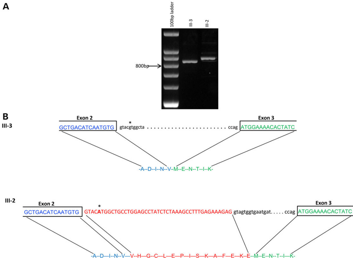
Figure 2. Partial analysis of ZC4H2 cDNA in family K9333. (A) RT-PCR of ZC4H2 mRNA prepared from individuals III-2 and III-3 in family K9333 using 4% agarose. (B) Sequence of ZC4H2 from individuals III-2 and III-3 flanking the exon 2/exon 3 boundary. The schematic shows how the insertion of 45 bp in III-2 results from the c.225 + 5G > A mutation. Bases in the transcripts are in capital letters. Red letters indicate intron 2 sequence. The mutation site is indicated with an asterisk.
