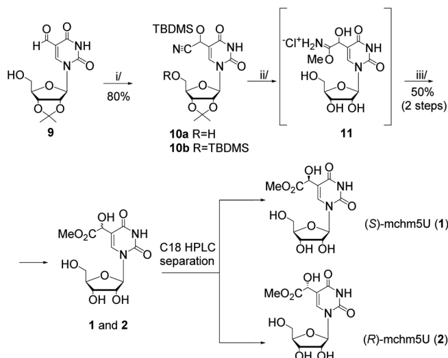
Scheme 2 The synthesis of ( S )- and ( R )-5-methoxycarbonylhydroxymethyluridine (1 and 2) starting with 5-formyluridine 9. Reagents and conditions: i/TBDMSCN, NEt 3 , CH 3 CN, rt, 2 h; ii/4 M HCl/MeOH, 5 °C, 2 h; iii/H 2 O, 5 °C, 2 h.
