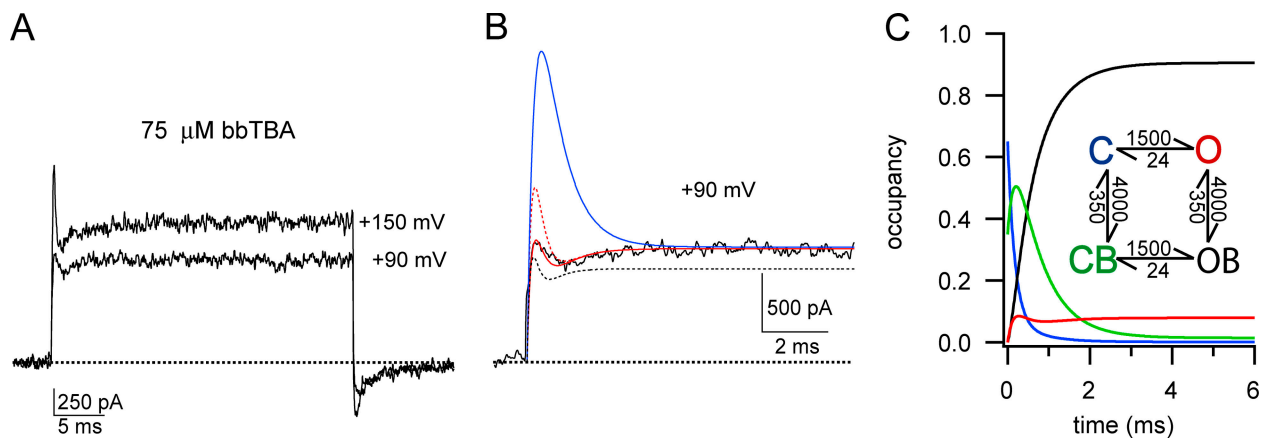
Figure 11. Blockade at high concentrations of bbTBA has three kinetic components. (A) Ionic currents (average of 10 sweeps) in the presence of 75 \mu\text{M} bbTBA at +90 or +150 mV. Holding potential was -80 mV. Triphasic block kinetics become more obvious at higher potentials; current rises during the first phase, then falls during the second phase, and finally rises again to steady-state levels during the third phase. (B) The current trace at +90 mV (+75 \mu\text{M} bbTBA) is shown on an expanded time scale. Smooth lines represent model predictions. The final state-independent model of bbTBA blockade (illustrated in C) was able to reproduce general kinetic and steady-state features of block (black dashed line). Model parameters were \alpha = 2330 s ^{-1} and \beta = 24 s ^{-1} for channel opening and closing, respectively (using single exponential fits to activation of control current at +90 mV and P_o = 0.99 , 1/\tau = \alpha + \beta and P_o = \alpha / (\alpha + \beta) ), K_d(0) = 9 \mu\text{M} , z\delta = 0.15 , and 50% channels initially in CB. Minor adjustment of these model parameters ( K_d(0) = 11 \mu\text{M} , z\delta = 0.15 , 35% channels initially in CB) and adding the assumption that bbTBA slows activation (from 2,330 to 1,500 s ^{-1} ) produced a better fit (solid red line). This adjusted state-independent model fits only when some fraction of channels are blocked at rest (compare with dashed red line where 100% channels start in C). Using the same adjusted parameters ( K_d(0) = 11 \mu\text{M} , z\delta = 0.15 , 35% CB, \alpha = 1500 s ^{-1} , \beta = 24 s ^{-1} ), the state-dependent model (e.g., Scheme 2) is clearly incompatible with the observed kinetics of block (solid blue line). Importantly, the state-dependent model was never able to reproduce triphasic block kinetics, even with extensive alteration of parameters (including starting up to 100% of channels in the blocked state). (C) Occupancy of the closed (C, blue), open (O, red), open blocked (OB, black), and closed blocked (CB, green) states over time illustrates the origin of triphasic block kinetics. Initial conditions for this occupancy plot modeling block by 75 \mu\text{M} bbTBA at +90 mV were 50% C + 50% CB; the same rate constants that were used for modeling the solid red line in B were used, as illustrated in the inset. Triphasic time-dependent block is a direct result of rapid population of blocked states prior to equilibration of the open state, in direct contrast to state-dependent models that require that the slow C to O transition be rate limiting for block. The triphasic kinetics of block observed at high concentrations of bbTBA strongly suggest that blockade is not state dependent.
