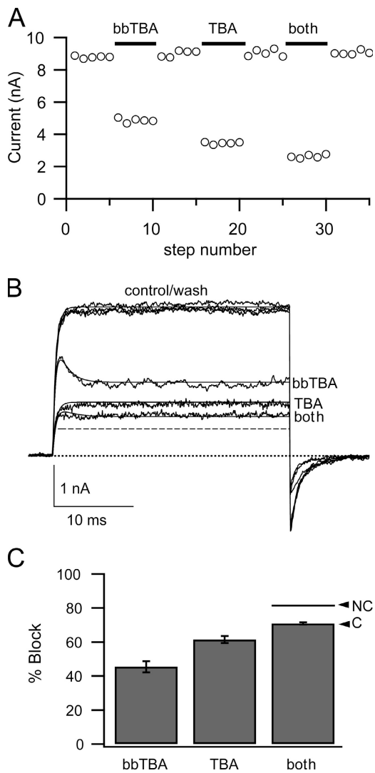
Figure 3. bbTBA behaves as a traditional pore blocker. (A) Ionic currents were sampled for 30 ms at +120 mV (from a holding potential of -80 mV) five times in each condition ( 100 \mu\text{M} internal \text{Ca}^{2+} or in the presence of 5 \mu\text{M} bbTBA, 1 \text{ mM} TBA, or both blockers together) in the order shown in the time course. (B) Each set of five sweeps was averaged to yield the average traces for this experiment in the absence and presence of the indicated blocker solutions. Percent block in each case was then calculated from these average sweeps (for this experiment: bbTBA, 51%; TBA, 65%; both, 72%). Smooth lines represent modeling of ionic current under each condition. For modeling, channel opening ( \alpha = 2254 \text{ s}^{-1} ) and closing ( \beta = 46 \text{ s}^{-1} ) rates were determined from a single exponential fit to the control data and assuming P_o \sim 0.98 , using 1/\tau = \alpha + \beta and P_o = \alpha/(\alpha + \beta) . Kinetics of TBA block were estimated from Li and Aldrich (2004): K_d(0 \text{ mV}) = 1 \text{ mM} and z\delta = 0.2 . bbTBA block was modeled using parameters for the final model ( K_d(0) = 9.9 \mu\text{M} and z\delta = 0.15 ). Currents in individual blockers were modeled with Scheme 3. Block by bbTBA + TBA was modeled using either a noncompetitive (Scheme 4, dashed line) or competitive (Scheme 5, solid line) model. Time dependence was drastically slowed in both cases, but the observed steady-state level of block is compatible only with a competitive model of block. (C) The average ( \pm SEM) percent block observed in three patches for bbTBA alone (46%), TBA alone (62%), or both blockers together (71%) follows exactly the predictions of a competitive model of blockade (71%). A noncompetitive model
