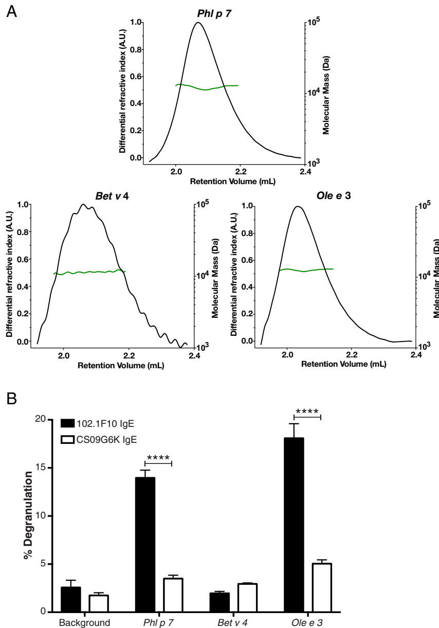
Fig. 2. Characterization of oligomeric state and basophil degranulation for the three polyclonal allergens. (A) Chromatograms of the RI signals for Phl p 7 , Bet v 4 , and Ole e 3 . The three proteins [in 25 mM Tris-HCl (pH 7.4) and 150 mM NaCl with 4 mM CaCl 2 ] were run over a Superdex 75 5/150 column (GE Healthcare) at a flow rate of 0.3 mL/min. The differential RI is shown in black (A.U., arbitrary units). The green lines across the protein elution volumes show the molecular masses of the proteins, indicating a monomeric state. (B) Basophil degranulation assay showing the percentage degranulation of RBL-SX38 cells sensitized with 102.1F10 IgE (black bars) and CS09G6K IgE (white bars) antibodies followed by stimulation with 5,000 ng/ \mu L of Phl p 7 , Bet v 4 , or Ole e 3 or with assay medium (background). Degranulation is expressed as a percentage of that induced by cell lysis. Bars represent the mean \pm SEM of three independent experiments. Statistical significance was determined by t test; **** P < 0.0001.
