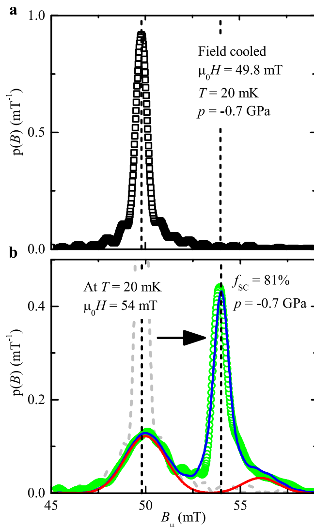
Figure 5. Vortex pinning in the SC phase of \text{CeCo}(\text{In}_{1-x}\text{Cd}_x)_5 , p = -0.7 GPa (field shift experiment).
