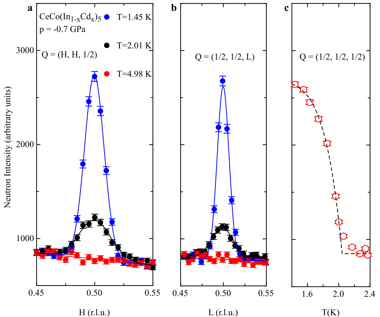
Figure 2. Scans in the reciprocal space of the neutron diffraction intensity of \text{CeCo}(\text{In}_{1-x}\text{Cd}_x)_5 , performed along the lines Q = (H, H, 1/2) in (a) and Q = (1/2, 1/2, L) in (b). Reciprocal lattice units (r.l.u.) are used as coordinates of the reciprocal space. The \text{CeCo}(\text{In}_{1-x}\text{Cd}_x)_5 sample has a doping x corresponding to a negative pressure of p = -0.7 GPa. (c) Temperature dependence of the neutron diffraction intensity measured at Q = (1/2, 1/2, 1/2) .
