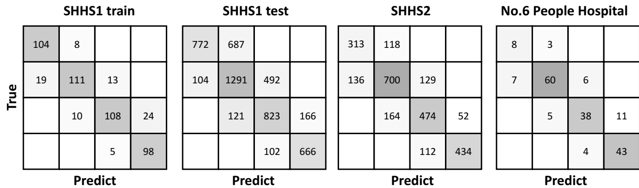
Figure 8 Confusion matrix for SDB severity classification based on computed AHI of four datasets (SHHS1 train, SHHS1 test, SHHS2 and No. 6 People Hospital).
