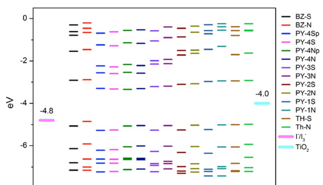
Fig. 3 Selected MOs energy levels (from HOMO–4 to LUMO+4) for the studied dyes at B3LYP/6-311+G(3df,3dp)/SMD level together with \text{TiO}_2 CB and \text{I}^-/\text{I}_3^- redox potential. p = planar structure.
