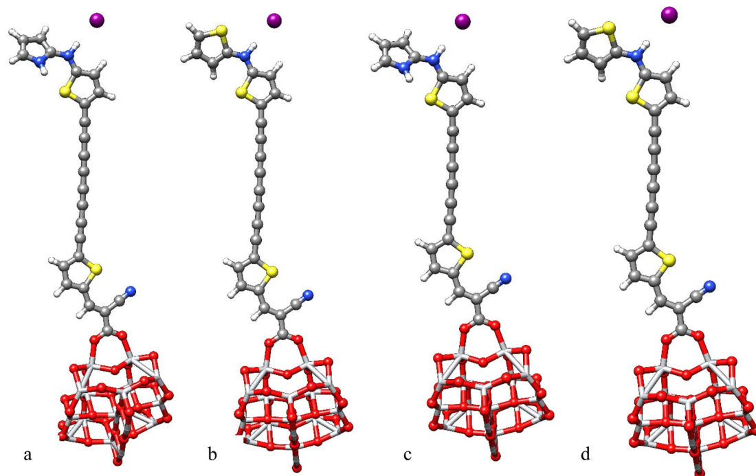
Fig. 9 Optimized geometries of I - -PY-4N@(TiO 2 ) 14 (a), I - -PY-4S@(TiO 2 ) 14 (b), I - -PY-3N@(TiO 2 ) 14 (c), I - -PY-3S@(TiO 2 ) 14 (d) at B3LYP-D3/6-31G(d)/LANL2DZ/SDDALL level.
