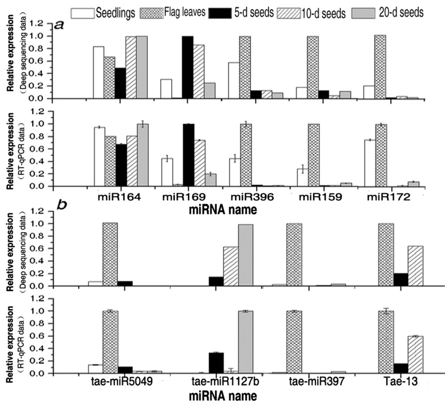
Figure 2 Comparison of the miRNA expression profiles determined by quantitative real-time RT-PCR (qPCR) and deep sequencing. a , known miRNAs; b , novel miRNAs and candidate miRNAs. In qPCR, UBQ was used as the internal reference gene, and the relative expression of each miRNA was calculated using a comparative C_T ( \Delta\Delta C_T ) method. The miRNA sample with the lowest C_T value that corresponds to the highest expression level was selected as the calibrator, in which the expression level was set as 1.0. The relative expression levels of the same miRNA in the other four samples were then normalised by comparing with the highest one in the tested tissues. Three independent biological replicates were performed in this experiment. For each sample, qPCR was performed in triplicate. Each column represents the mean of three samples, and error bars represent the standard deviation. In deep sequencing technology, read counts for each miRNA in one sample were normalised to reads per million of total miRNA reads (RPM). The relative expression of each miRNA was calculated by setting the highest RPM of each miRNA across the five samples as 1.0, and the relative expression of the same miRNA in the other four samples was its RPM divided by the highest RPM.
