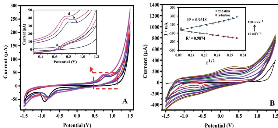
Fig. 3 (A) Cyclic voltammograms of (a) bare SPE (b) SPE/PPy, (c) SPE/PPy/TA and (d) SPE/PPy/TA/CTAB. Scan rates: 0.1 \text{ V s}^{-1} . Inset plot shows an enlarged view of the anodic peak. (B) Cyclic voltammograms of PPy/TA/CTAB modified electrode with different scan rate. Inset plot shows oxidation and reduction peaks against square root of scan rate. All was done in PBS buffer solution (pH 7.0).
