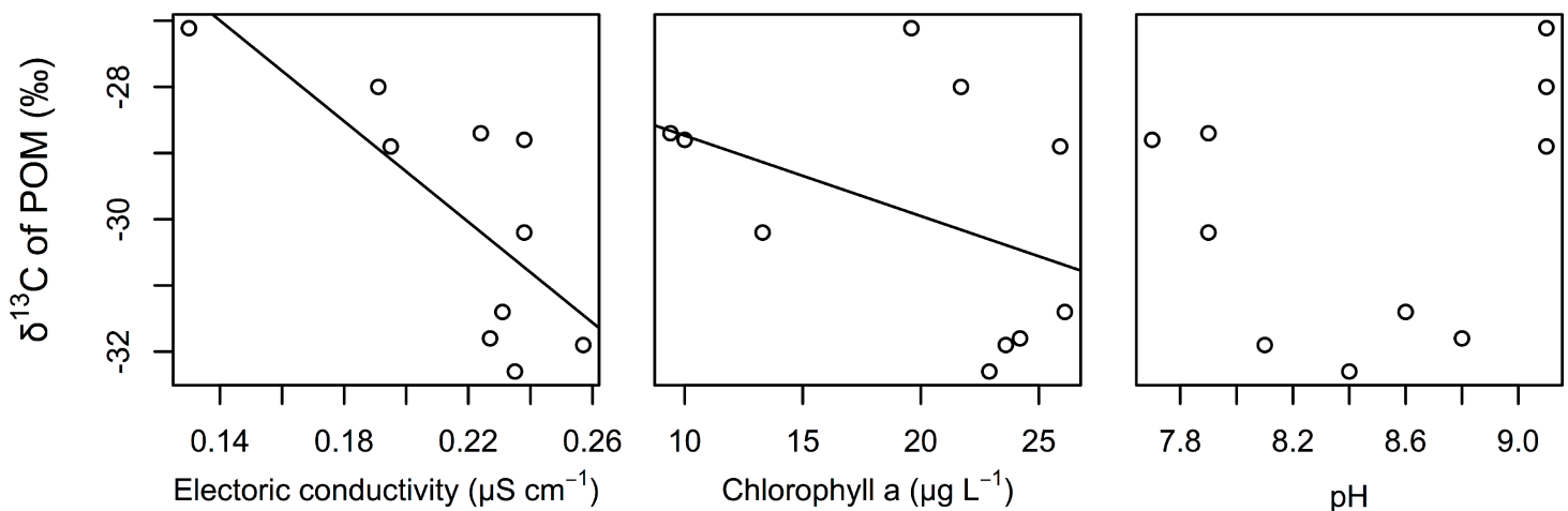
Figure 3 Relationships between the \delta^{13}C values of POM and electrical conductivity, chlorophyll a , and pH of the surface water. The lines are regression lines obtained using the best GLM.
