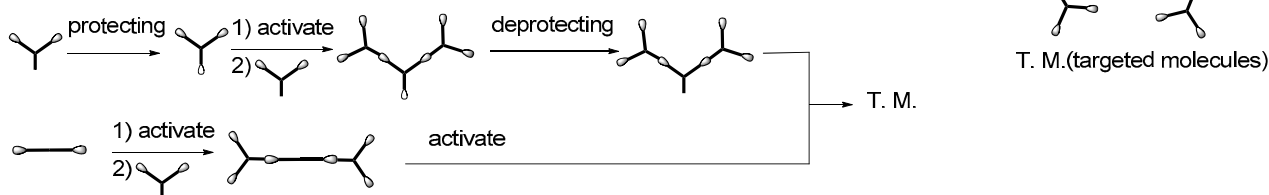
Scheme 1. Preparation of dendrimers by the convergent, divergent, and combined approaches.
