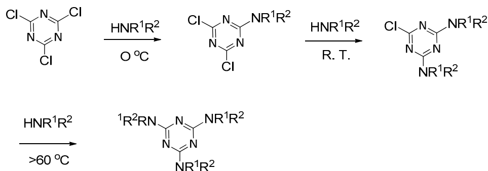
Scheme 2. Reaction of amines with cyanuric chlorides at different temperatures.
