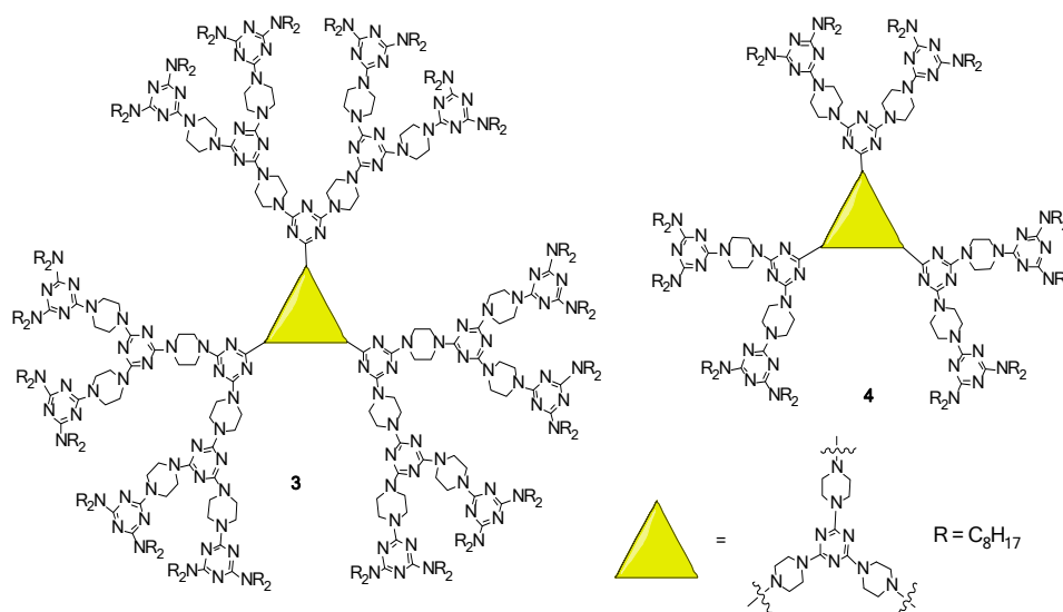
Figure 2. Structures of dendrimers ( 3 ) and ( 4 ) with C_3 -symmetry.
