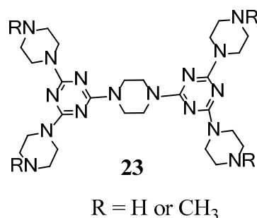
Figure 13. Structure of molecule ( 23 ).
