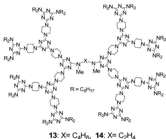
Figure 8. Structures of dendrimers (13) and (14).
