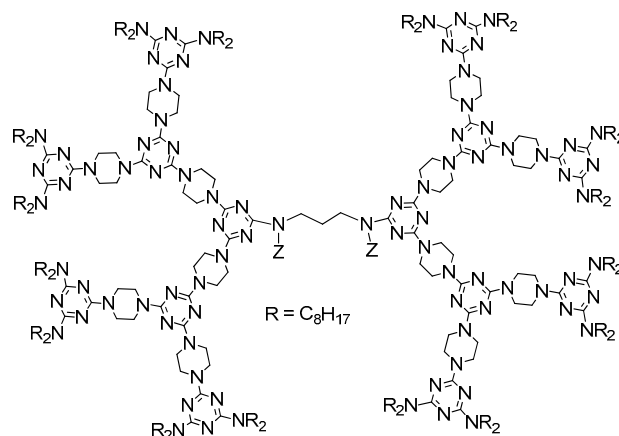
15: Z = CH 2 -C 6 H 5 , 16: Z = CH 2 -C 6 H 4 CN
