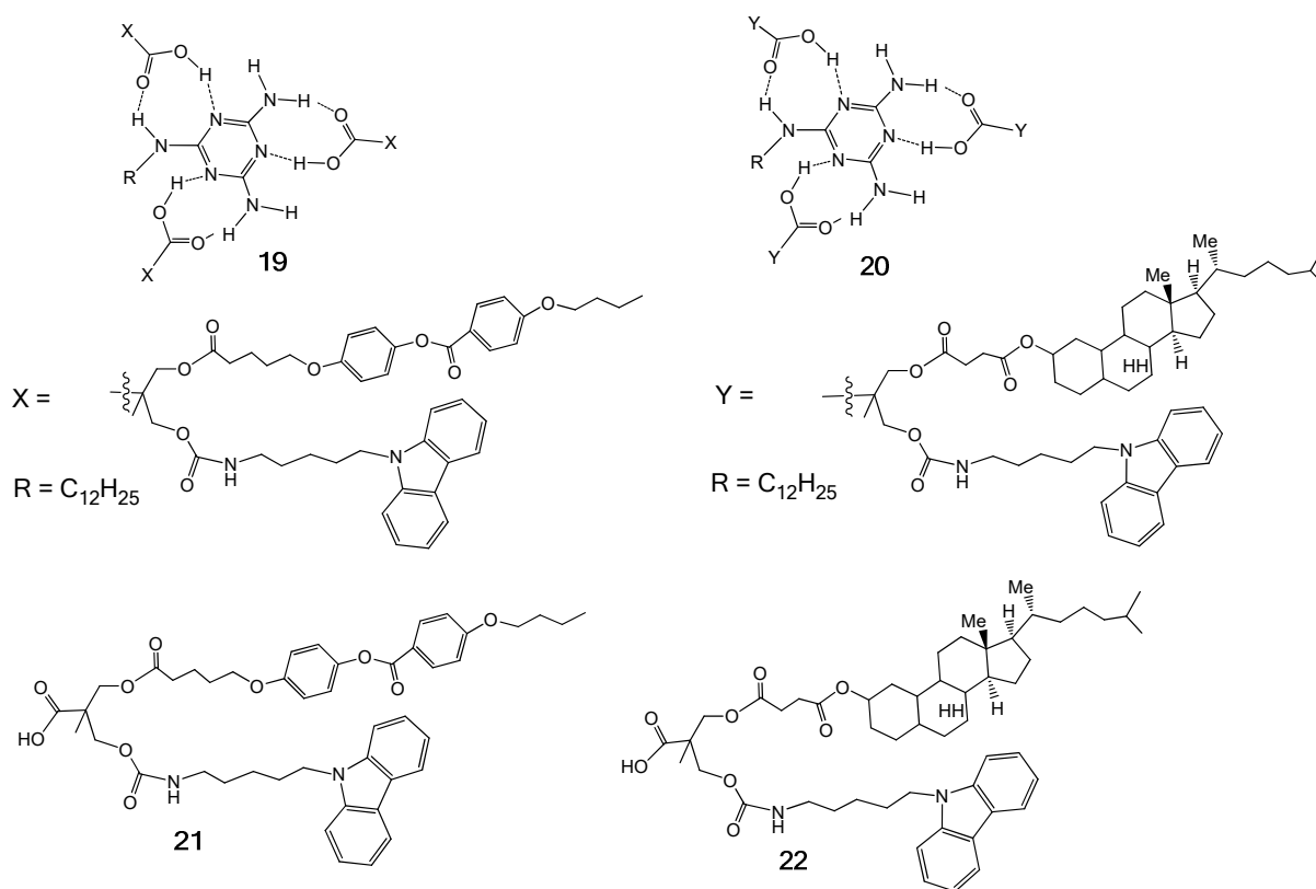
Figure 12. Structures of dendrimers (19) and (20) and dendrons (21) and (22).
