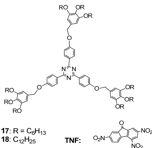
Figure 11. Structures of dendrimers ( 17 ) and ( 18 ).
