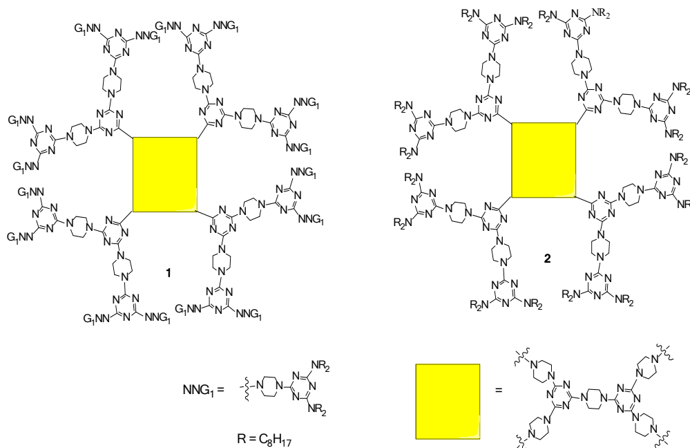
Figure 1. Structures of dendrimers ( 1 ) and ( 2 ) with C_2 -symmetry.
