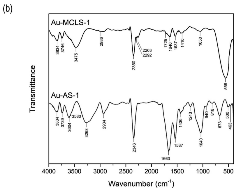
Fig. 6 Analysis and comparison of Au-MCLS-1 and Au-AS-1 compounds: (a) corresponding organosulfur compounds of AS extract obtained from 1 H NMR spectral features of Au-AS-1 nanoparticle system in comparison to the 1 H NMR spectra of Au-MCLS-1 as inset, and (b) FTIR spectral peaks corresponding to functional groups of Au-MCLS-1 before and after functionalization with AS extract to produce Au-AS-1. Differences in peak positions and features imply functionalization via substitution/displacement from Au-MCLS-1 to Au-AS-1.
