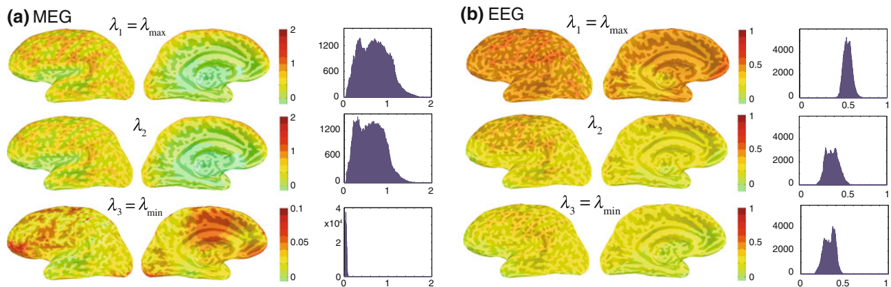
Fig. 2 Distribution of the sensitivity to three orthogonal source components at each location on the cortex, indicated by the singular values ( \lambda_{k,1} = \lambda_{k,max} , \lambda_{k,2} , \lambda_{k,3} = \lambda_{k,min} ) of the dipole gain matrix \mathbf{A}_k for MEG (a) and EEG (b). Note that for MEG, the color scales in the
