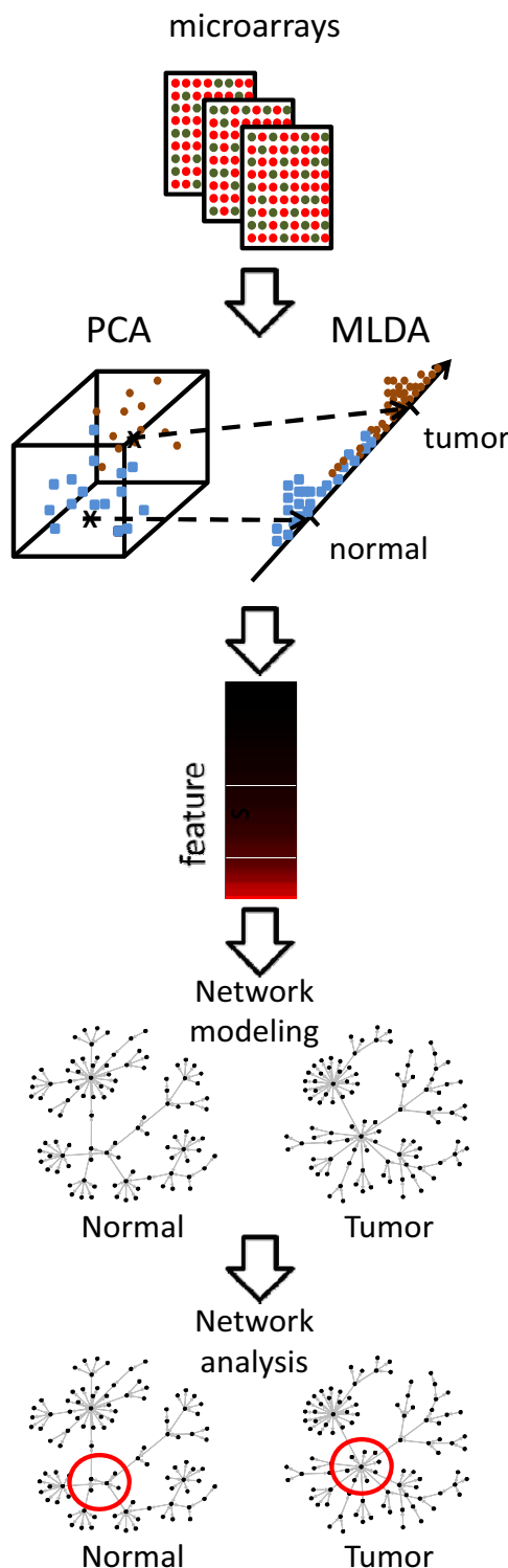
Figure 1 A pictorial scheme of the combination of PCA+MLDA and dependence network analysis for two populations (normal and tumoral prostatic tissues).
