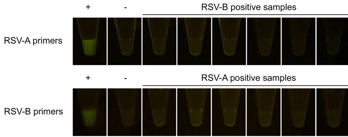
Supplementary Figure S1. The representative results of each set of primers when used against the other subtype. RT-RPA + CRISPR using RSV-A primers on RSV-B targets, and vice versa.
