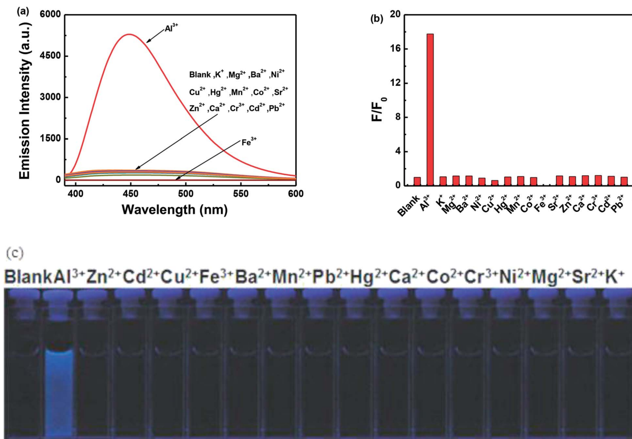
Fig. 4 Changes in the fluorescence of 10 induced by the addition of various metal ions (10.0 equiv.) in methanol ( 2.0 \times 10^{-5} \text{ mol L}^{-1} ): (a) emission spectral changes; (b) emission intensity changes; and (c) photograph of the change in fluorescence.
