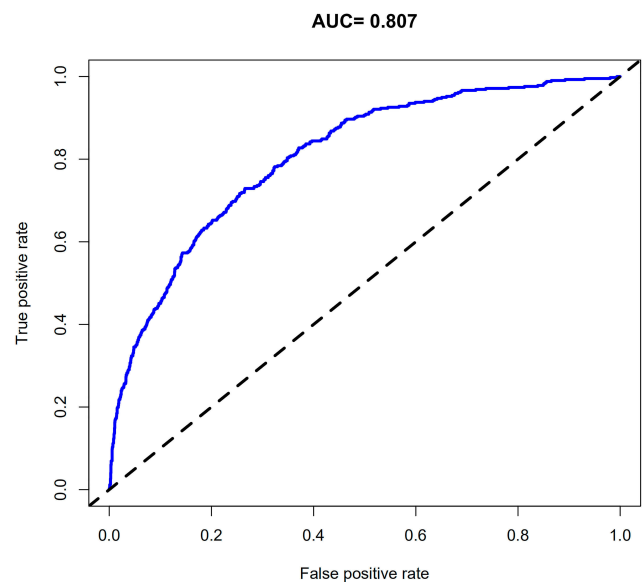
Figure 7 The pooled AUC of the ROC curve.
