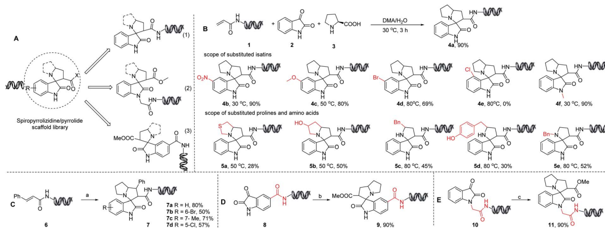
Fig. 3 On-DNA three-component cyclization using three DNA-tagging points. (A) Three types of DNA-tagged spiroprolrolizidine centered modes. (B) Optimization of on-DNA three-component cyclization from acrylamide linked DNA oligonucleotides. Scope of substituted isatins, prolines and amino acids. (C) on-DNA reactions from DNA-linked 6. (a) Isatin (200 equiv.), proline (300 equiv.), 80 °C, 3 h. (D) On-DNA cyclization reaction from DNA-linked 8. (b) Acryl ester (200 equiv.), proline (200 equiv.), rt, 3 h. (E) On-DNA cyclization reaction from DNA-linked 10. (c) Acryl ester (200 equiv.), proline (200 equiv.), rt, 3 h. Conversions determined by LCMS.
