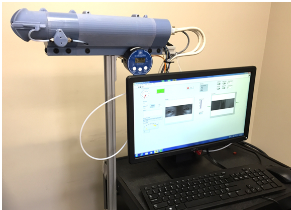
FIGURE 1. Blink reflexometer housing unit and software interface. Tubing connected to the left end of the housing unit delivers a puff of compressed air to the subject's eyes.
