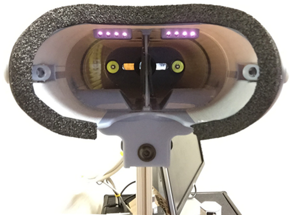
FIGURE 2. The housing unit has a center barrier to prevent inadvertent stimulation of the contralateral eye. Two arrays of IR LEDs provide scene illumination.
