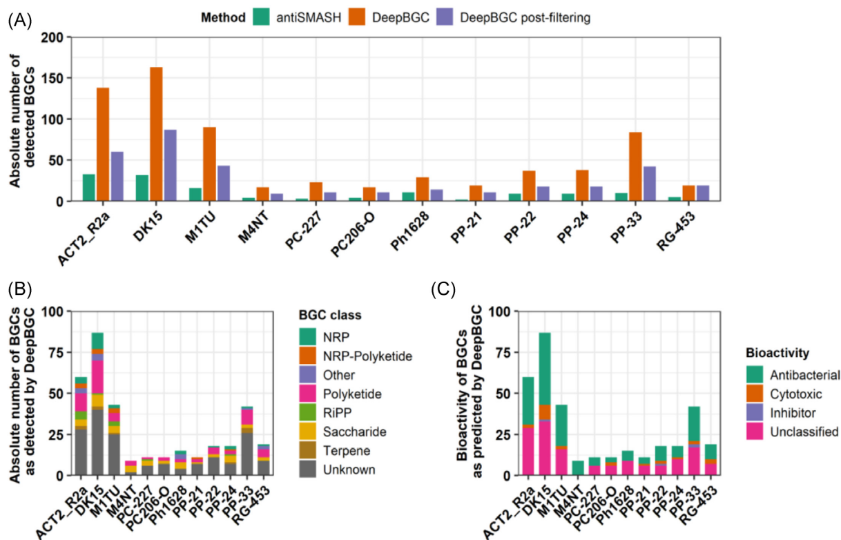
Figure 4. Summary of biosynthetic gene clusters (BGCs) and proposed activity as predicted by DeepBGC. (A) Comparison of BGCs as detected by the two tools utilized, including a stringent filtering step using DeepBGC to remove low-quality hits. Breakdown of the (B) classes of BGCs and (C) the predicted biological activity of proposed BGCs as detected by DeepBGC.
