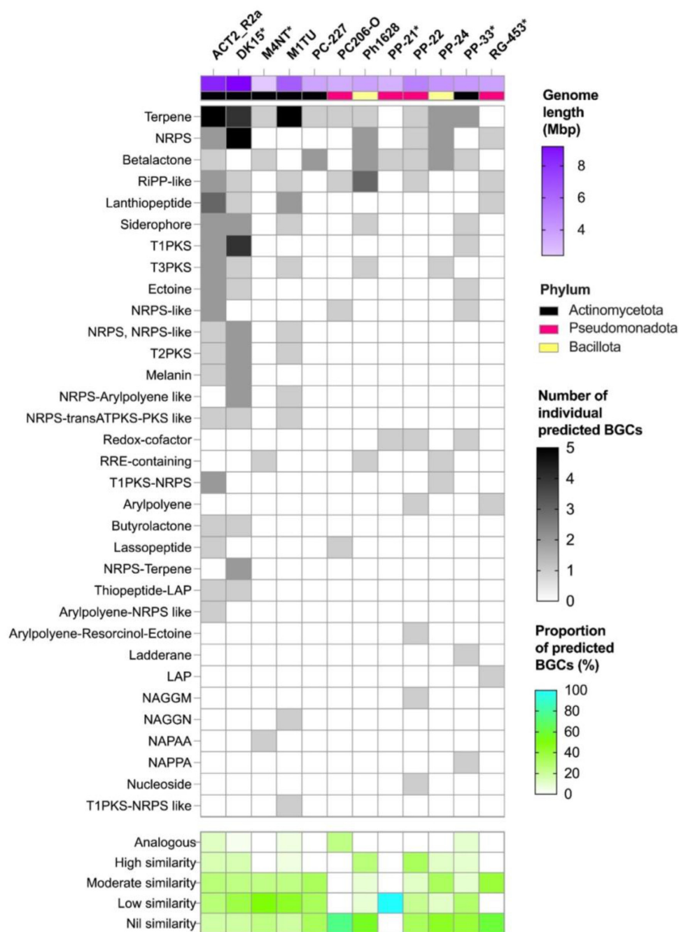
Figure 3. Predicted biosynthetic gene clusters (BGCs) from sponge-associated bacterial genomes. Summary of the predicted BGCs, and the proportion of BGCs classified based on similarity to known BGCs. Strains are ordered from highest to lowest number of predicted BGCs going from the left to the right. For a detailed breakdown of all predicted BGCs refer to Table S2. (RiPP, ribosomally synthesized post-translationally modified; PKS, Polyketide synthase; NRPS, non-ribosomal peptide synthase; *, potentially novel species).
