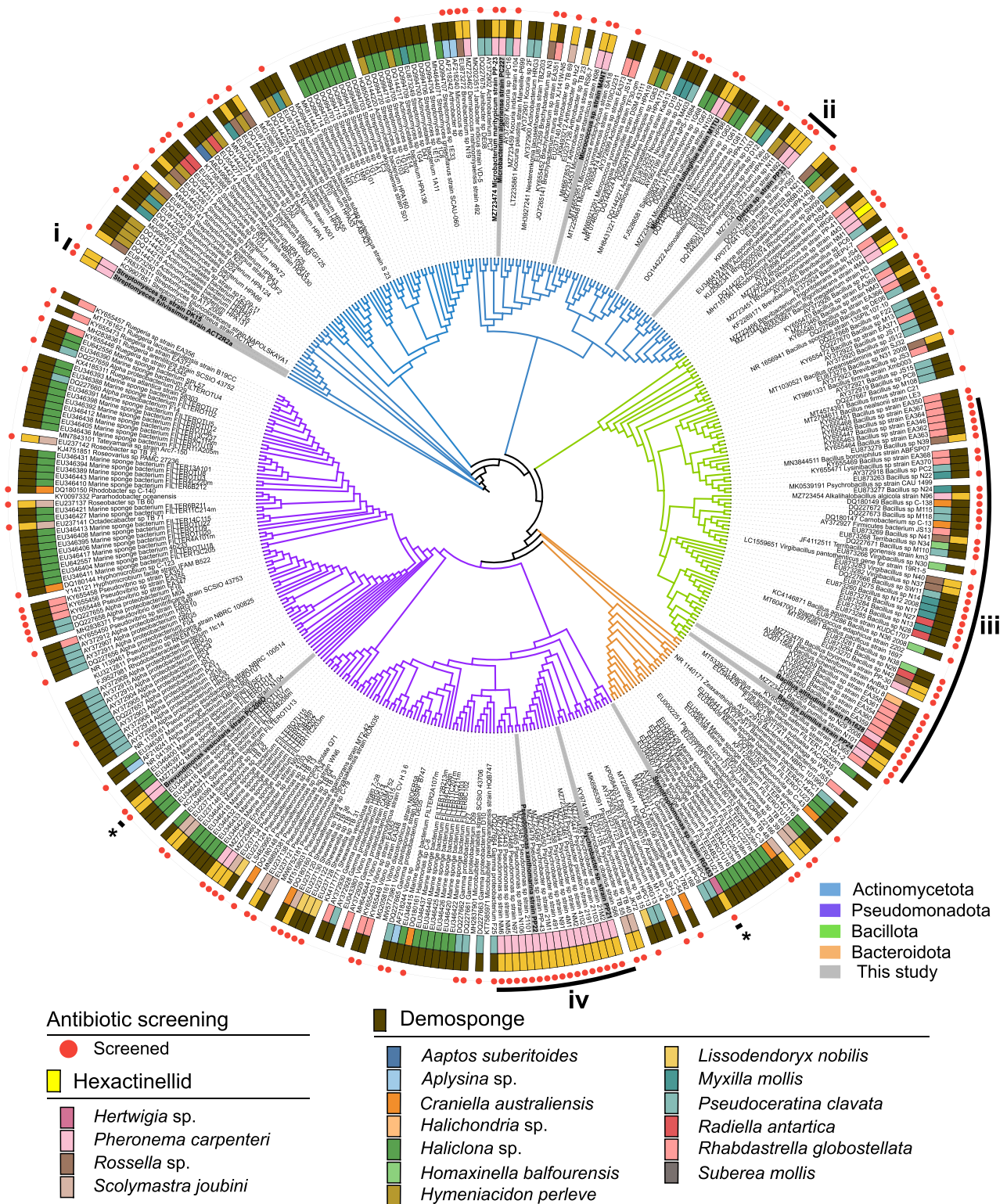
Figure 2. Maximum likelihood phylogenetic tree of 16S rRNA gene sequences from cultivable sponge-associated bacteria showing that antibiotic producers are phylogenetically diverse across all classes and species of sponge. Cultivable sponges presented here include reference organisms, a selection of bacteria cultivated in this study that display antimicrobial activity and those from published studies (Lafi et al. 2005, Kim and Fuerst 2006, Jiang et al. 2007, Mangano et al. 2008, Zhang et al. 2008, Siphema et al. 2011, Xin et al. 2011, Bibi et al. 2020, Koch et al. 2021). The outer ring represents whether organisms were screened for antibiotic activity in the published study, the middle ring the class of the sponge bacteria were cultivated, and the inner ring the taxonomy of the sponge. Regions of interest are marked numerically (i-iv). Sequence names as part of this study are labelled first with an NCBI accession number and the taxonomic classification and isolate name of the bacteria from the original study (see Supplementary Table 2). Bacterial isolates investigated in this study are labelled with their unique isolate name in bold and a grey strip.
