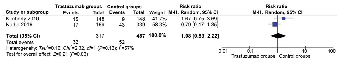
Figure 7 Forest plot: CNS metastasis.
