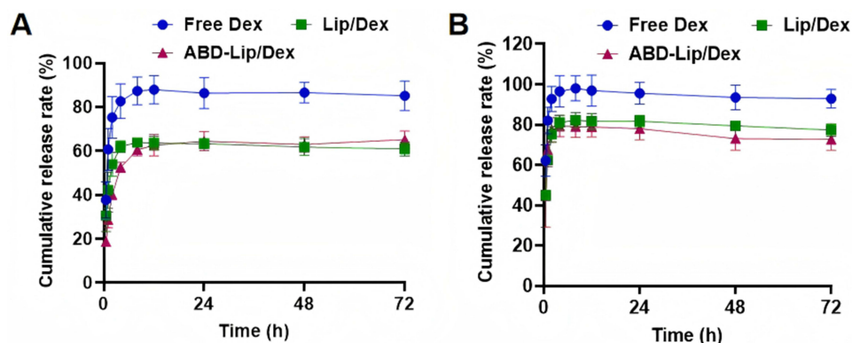
Figure 3 Drug release of the liposomes in vitro. (A) Dialysis-based assays of drug release in vitro in PBS. (B) Dialysis-based assays of drug release in vitro in PBS containing 10% (v/v) fetal bovine serum. Results are the mean \pm SD of three independent batches.
