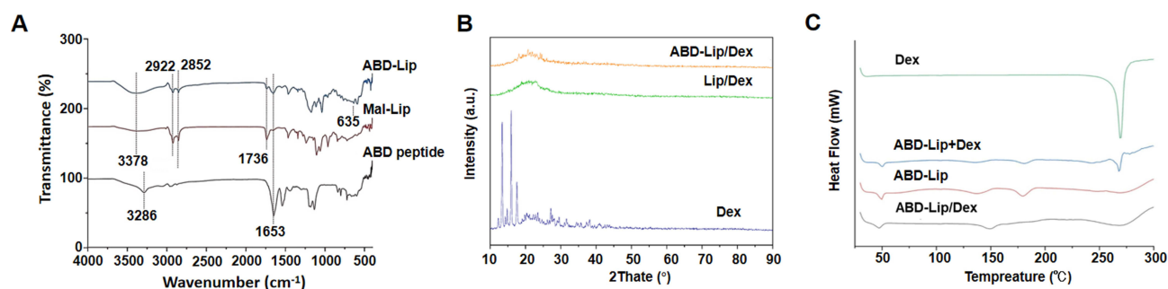
Figure 2 Characterization for the structure of liposomes. (A) Fourier transform infrared spectroscopy. (B) X-ray diffraction analysis. (C) Differential scanning calorimetry. Results are the mean ± SD of three independent batches.
