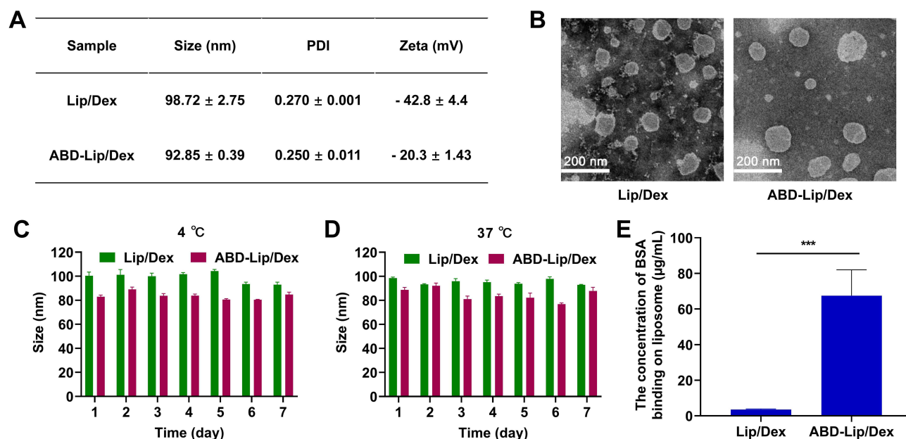
Figure 1 Characterization of liposomes loaded with Dex and either unmodified (Lip/Dex) or modified with the “albumin-binding domain” peptide (ABD-Lip/Dex). (A) Diameter, polydispersity index and zeta potential, based on dynamic light scattering. Results are the mean ± SD of three independent batches. (B) Transmission electron micrographs. (C) Liposome diameter during storage at 4 °C. (D) Liposome diameter during storage at 37 °C. (E) Quantitation of the binding of FITC-conjugated bovine serum albumin to the surface of liposomes in vitro. Results are the mean ± SD of three independent batches. ***, P < 0.001 .
