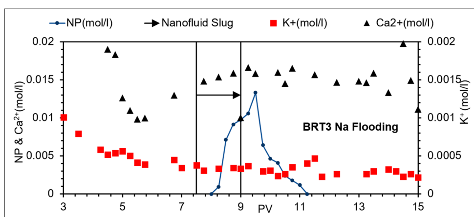
Figure 9. Effluent ion composition, BRT3 Na brine flooding.
