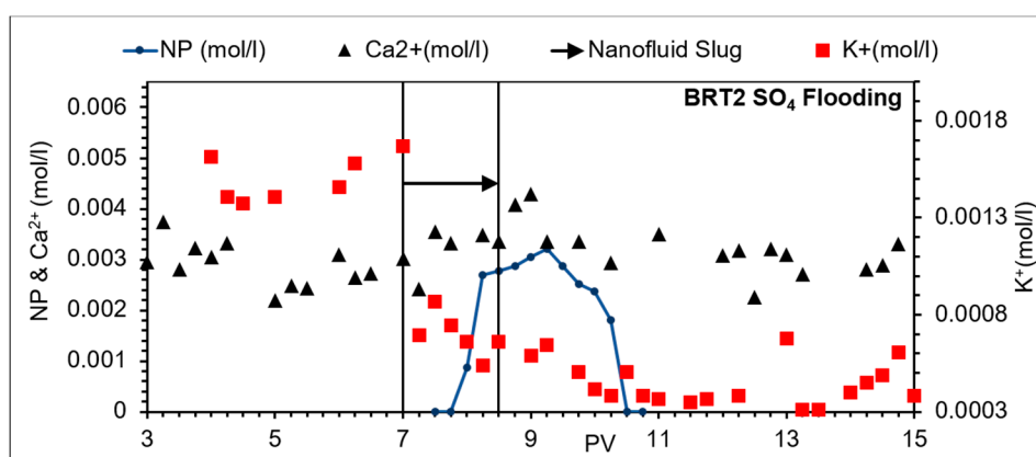
Figure 8. Effluent ion composition, BRT2; SO 4 brine flooding.
