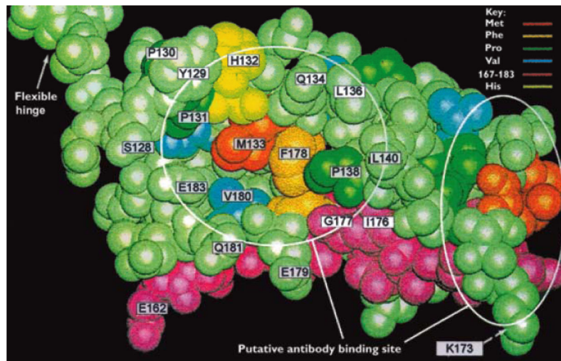
Figure 1. Three-dimensional structure of the PDC-E2 inner lipoylated domain based on published NMR structure 16
