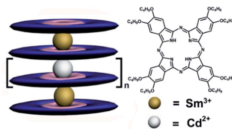
Scheme 1 Schematic molecular structures of tris- to hexakis(phthalocyaninato) metal complexes \{[(\text{Pc}^*)\text{Sm}][(\text{Pc}^*)\text{Cd}_n(\text{Pc}^*)_n][\text{Sm}(\text{Pc}^*)]\} ( n = 0-3 ) (3-6).
