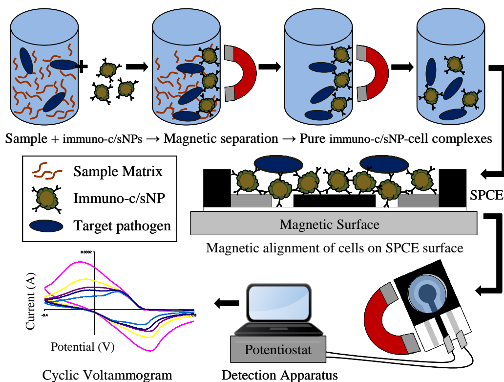
Figure 2. Immunomagnetic separation from sample matrix, magnetic alignment on SPCE surface, and electrochemical detection of B. cereus and E. coli O157:H7 cells.
