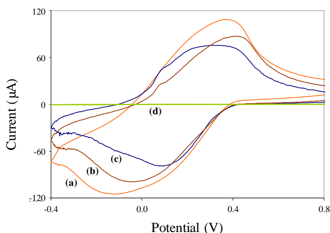
Figure 3. Cyclic voltammograms of (a) 1 mg/mL c/sNPs; (b) 1 mg/mL immuno-c/sNPs; (c) 0.1 mg/mL polyaniline nanoparticles, each suspended in 0.1 M HCl solution; and (d) 0.1 M HCl solution alone.
