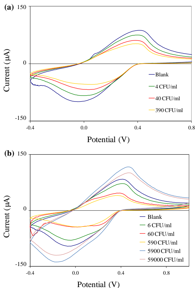
Figure 5. Cyclic voltammograms of immuno-c/sNP-cell solutions: (a) B. cereus cell concentrations ranging from 4 to 3.9 \times 10^2 CFU/mL; and (b) E. coli O157:H7 cell concentrations ranging from 6 CFU/mL to 5.9 \times 10^4 CFU/mL.
