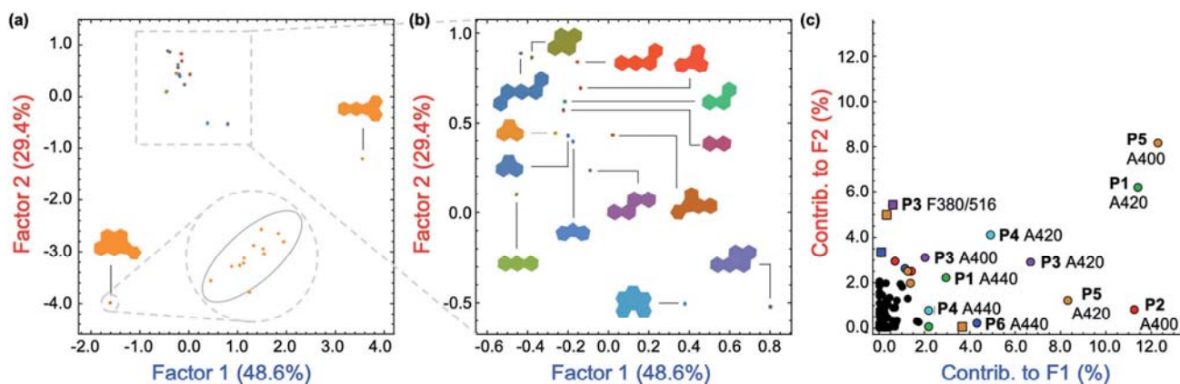
Fig. 4 (a) Two-dimensional plot of the LDA scores for the attempted differentiation of 16 PAHs with P1–P6. The plot was generated using 114 instrumental variables and captures 78.0% of the total information in the raw dataset. The inset shows a representative tight intra-cluster spacing of 12 replicate samples of indeno[1,2,3- cd ]pyrene ([PAH] = 500 \mu\text{M} ). (b) Zoomed-in LDA scores plot from (a) for 14 PAHs, displaying low inter-cluster spacing between those PAHs. (c) LDA loadings plot for the differentiation of 16 PAHs shown in (a), indicating the relative contributions of each instrumental variable to the first two LDA factors. Colored squares: contributions from fluorescence measurements. Colored circles: contributions from absorbance measurements.
