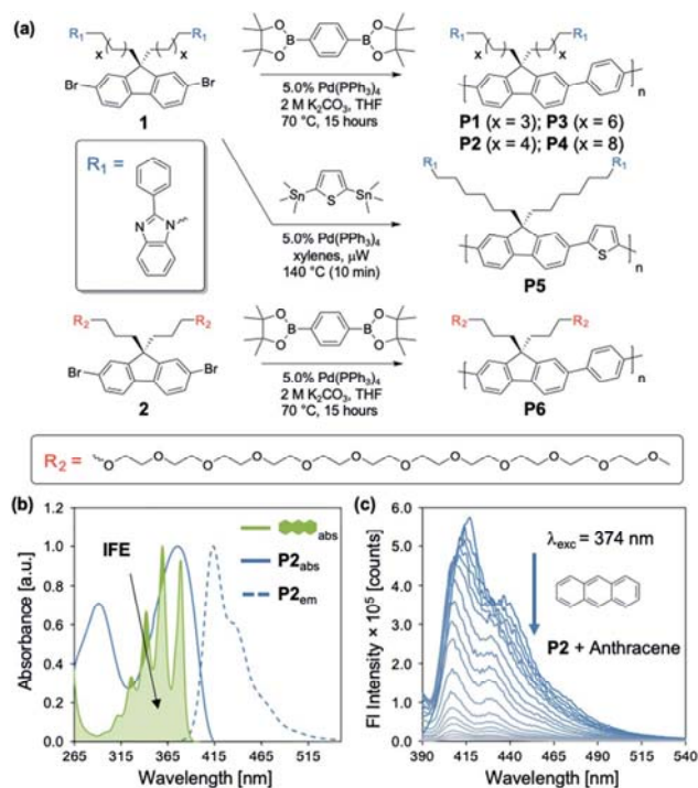
Fig. 1 (a) Synthesis of P1–P6. (b) Normalized excitation and emission spectra of P2 overlaid with normalized anthracene absorption ([anthracene] = 10 μM; [P2] = 15 mg L -1 ), providing the basis for an IFE. (c) Fluorescence spectra of P2 (15 mg L -1 ) upon titration with anthracene (0–9.4 mM) in N,N -dimethylformamide (DMF) (λ exc = 374 nm).
